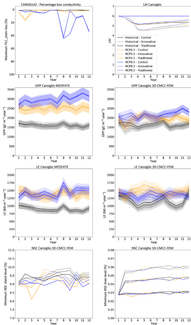
Fig. 4. Comparative analysis between models output at the Cansiglio site. The top-left panel displays the PLC_{stem} as modelled by MEDFATE, while the top-right panel shows the modelled LAI for 3D-CMCC-FEM (and used by MEDFATE). The middle-up panels (left and right) present annual GPP ( gC\cdot m^{-2}\cdot year^{-1} ) as modelled by the MEDFATE and 3D-CMCC-FEM, respectively. The middle-down panels (left and right) depict annual LE ( MJ\cdot m^{-2}\cdot year^{-1} ) modelled by the MEDFATE and 3D-CMCC-FEM, respectively. The bottom panels (left and right) depict the annual minimum of NSC concentration (%) at the stand and tree level, respectively, as modelled by the 3D-CMCC-FEM. Different plot management strategies are represented by distinct line styles: solid lines for 'Control' plots ('no management'), dotted lines for 'Innovative' plots, and dashed lines for 'Traditional' plots (Shelterwood). Climate scenarios are indicated by line colours: black for 'Hist' climate data (2010–2022), orange and blue for RCP4.5 and RCP8.5 climate (2059–2070), respectively.
