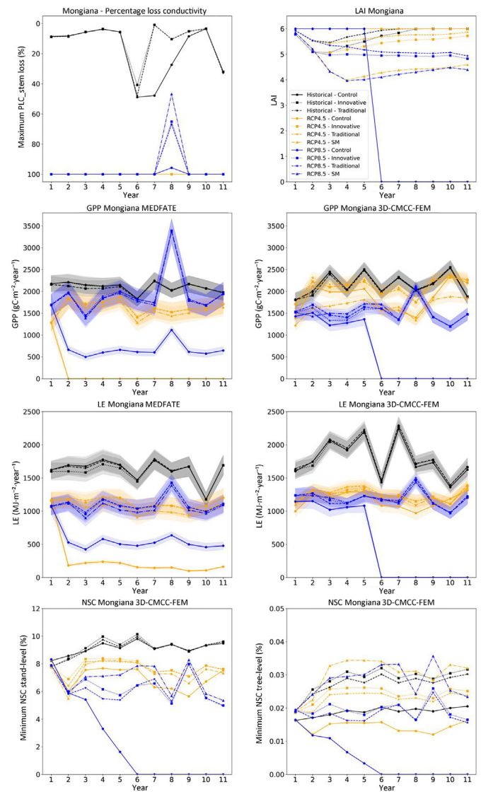
Fig. 5. Comparative analysis between models output at the Mongiana site. The top-left panel displays the percent loss of PLC_{stem} as modelled by MEDFATE while the top-right panel shows the modelled LAI for 3D-CMCC-FEM (and used by MEDFATE). The middle-up panels (left and right) present annual GPP ( gC\cdot m^{-2}\cdot year^{-1} ) as modelled by the MEDFATE and 3D-CMCC-FEM, respectively. The middle-down panels (left and right) depict annual LE ( MJ\cdot m^{-2}\cdot year^{-1} ) modelled by the MEDFATE and 3D-CMCC-FEM, respectively. The bottom panels (left and right) depict the annual minimum of NSC concentration (%) at the stand and tree level, respectively, as modelled by the 3D-CMCC-FEM. Different plot management strategies are represented by distinct line styles: solid lines with circles for 'Control' plots ('no management'), dotted lines with squares for 'Innovative' plots, dashed lines with stars for 'Traditional' plots (Shelterwood) and dash-dotted lines with triangles for 'SM' management. Climate scenarios are indicated by line colours: black for 'Hist' climate data (2010–2022), orange and blue for RCP4.5 and RCP8.5 climate (2060–2070), respectively.
