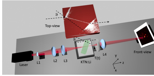
Fig. 1. Anti-diffraction setup. A He-Ne laser operating at 633 nm is enlarged through lenses L1 and L2 and focused down to an 8\ \mu\text{m} spot at the input facet of the KTN:Li sample, rotated with the respect to the propagation axis z by a variable angle \theta and brought through a temperature cycle T(t) . (Front-view) The input and output facets are imaged through lens L4 onto a CCD camera. (Top-view) Scattered light is captured above the sample and imaged, through a microscope, onto a second CCD camera.
