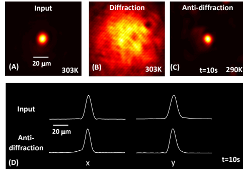
Fig. 3. Weak anti-diffraction for T_D = 286\text{K} . The input 7.8\text{ }\mu\text{m} beam (a) diffracts as in the previous case (b) and shrinks to 7\text{ }\mu\text{m} after 10 s (c). (d) Profiles of input and anti-diffracting beams (at t = 10\text{s} ).
