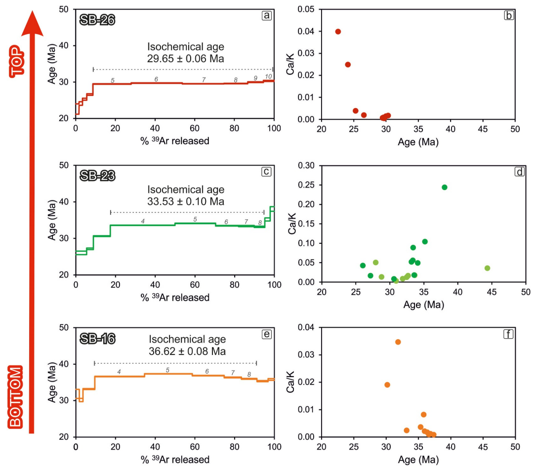
Figure 8. ^{40}\text{Ar}/^{39}\text{Ar} age spectra with obtained mean weighted age and Ca/K versus age diagrams for orthogneiss SB-26 (a, b), SB-23 (c, d) and SB-16 (e, f). The dated fraction size has been reported for each sample. All uncertainties are 1 \sigma error.
