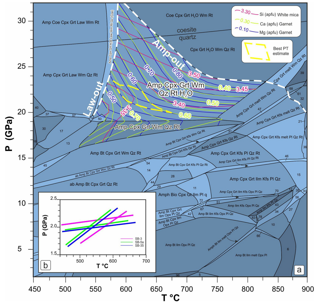
Figure 6. Isochemical phase diagram calculated using the bulk composition of sample SB5. Isopleths for Si in white mica, Ca and Mg in garnet are reported in the stability field of the peak equilibrium phase assemblage. Phase assemblages not reported in full are as follows: (5) Amp, Bt, Ilm, Opx, Pl, H 2 O; (6) Amp, Ilm, melt, Opx, Pl; (10) Amp, Ilm, Kfs, melt, Opx, Pl; (11) Amp, Bt, Cpx, Grt, Ilm, Kfs, Pl, Qz; (12) Amp, Cpx, Grt, Ilm, Kf, Pl, Qz; (13) Amp, Cpx, Grt, Wm, Qz; (14) ab, Amp, Bt, Cpx, Grt, Kfs, Qz, Rt; (15) Amp, Cpx, Grt, Ilm, Kfs, melt, Pl, Qz; (16) Amp, Cpx, Grt, Wm, Rt; (17) Amp, Cpx, Grt, Wm, Qz, Rt, Zo; (18) Amp, Cpx, Grt, melt, Pl, Rt; (21) Amp, Cpx, Grt, Kfs, melt, Pl, Rt; (29) Amp, Bt, Cpx, Ilm, Pl, Rt, Qz; (30) Amp, Cpx, Grt, Wm, Kfs, Q, Rt; (31) Amp, Cpx, Grt, Kfs, Wm, Qz, Rt; (32) Amp, Cpx, Grt, Kfs, melt, Rt; (35) Amp, Cpx, Ilm, Kfs, melt, Pl, Q; (37) Amp, Cpx, Grt, Law, Wm, Rt, Zo; (39) Cpx, Grt, melt Wm, Rt; (40) Amp, Cpx, Grt, Law, Wm, Rt; (42) Amp, Bt, Cpx, Ilm, Kfs, Opx, Pl, Qz; (43) Amp, Ilm, Kfs, melt, Pl, Qz; (45) Amp, Bt, Cpx, Grt, Ms, Q, Rt; (46) Amp, Cpx, Grt, Ilm, Kfs, melt, Pl, Q, Rt; (47) Amp, Cpx, Grt, Kfs, melt, Wm, Q, Rt; (50) Amp, Cpx, Grt, H 2 O, Wm, Q, Rt; (54) ab, Amp, Bt, Cpx, Grt, Kfs, Wm, Q, Rt; (55) Amp, Cpx, Ilm, Kfs, melt, Opx, Pl, Q; (57) Amp, Cpx, Grt, Law, Wm, Q, Rt, Zo; (60) Amp, Cpx, Grt, Ilm, Kfs, melt, Opx, Pl, Qz; (61) Amp, Cpx, Grt, Kfs, melt, Wm, Rt; (63) Amp, Bt, Ilm, Kfs, Pl, Qz; (66) Amp, Bt, Grt, Ilm, Kfs, melt, Opx, Pl; (67) Amp, Bt, Grt, Ilm, Kfs, Opx, Pl, Qz; (68) Amp, Cpx, Grt, melt, Wm, Rt; (70) Amp, Cpx, Ilm, Kfs, Opx, Pl, Qz; (72) Amp, Bt, Cpx, Grt, Ilm, Kfs, Opx, Pl, Qz; (74) Amp, Cpx, Grt, H 2 O, Wm, Qz, Rt, Zo; (78) Amp, Bt, Ilm, Kfs, melt, Pl, Qz; (96) Amp, Bt, Ilm, Pl. (b) PT estimates calculated with the Krogh Ravna (2000) and the Krogh Ravna and Terry (2004) geothermobarometers for the equilibrium phase assemblage Wm 2 + Cpx 1 + Grt 2 .
