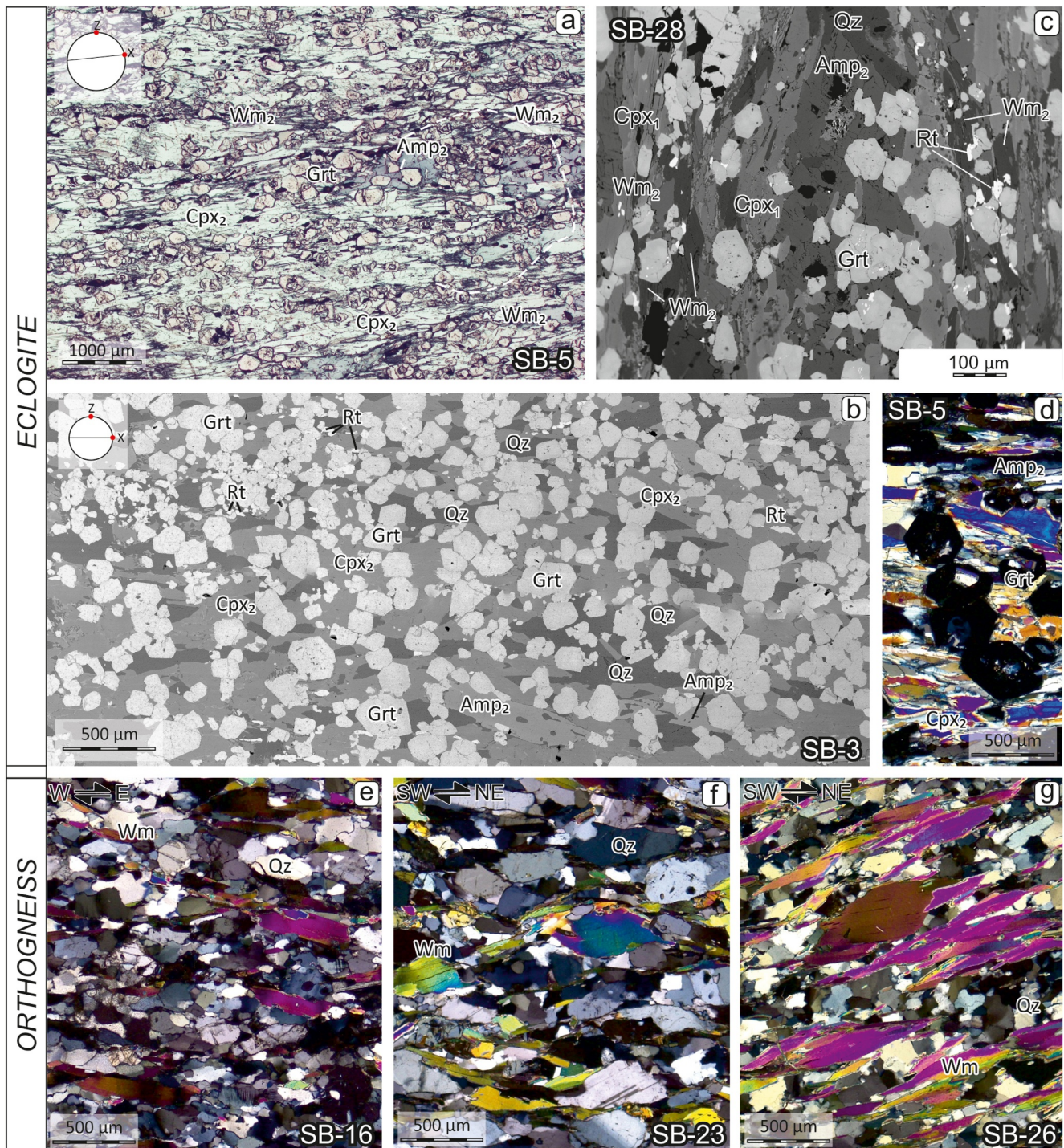
Figure 3. Photomicrographs of San Bernardino eclogites and orthogneisses. (a) Eclogite sample showing the main foliation made of Cpx 1 , Amp 2 and Wm 2 surrounding Grt porphyroblasts (parallel polars). (b) BSE panorama of eclogite characterized by a main foliation of Cpx 1 , Amp 2 and Wm 2 . (c) BSE image of a large Amp 2 porphyroblasts syn-kinematic to the eclogitic foliation. Garnet porphyroblasts, when having an aspect ratio that differs from 1:1, also appear elongated along the foliation. (d) Cross-polars photo of garnet porphyroblasts within the eclogite, containing inclusions of Wm and Amp. (e), (f) and (g) orthogneiss samples dated by 40 Ar/ 39 Ar method from bottom to top of the San Bernardino Shear Zone. In (e) the older foliation is still evident, whereas is fully overprinted in (g). The mineral abbreviations are as follows: Amp: amphibole; Ap: apatite; Bt: biotite; Cal: calcite; Chl: chlorite; Cpx: clinopyroxene; Czo: clinozoisite; Dol: dolomite; Grt: garnet; Ilm: ilmenite; Kfs: K-feldspar; Qz: quartz; Pg: paragonite; Pl: plagioclase; Rt: rutile; Ttn: titanite; Wm: white mica; Zr: zircon.
