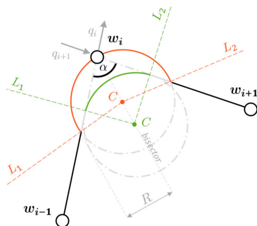
Figure 13. Orbit geometry and path planning in transition scenario.
