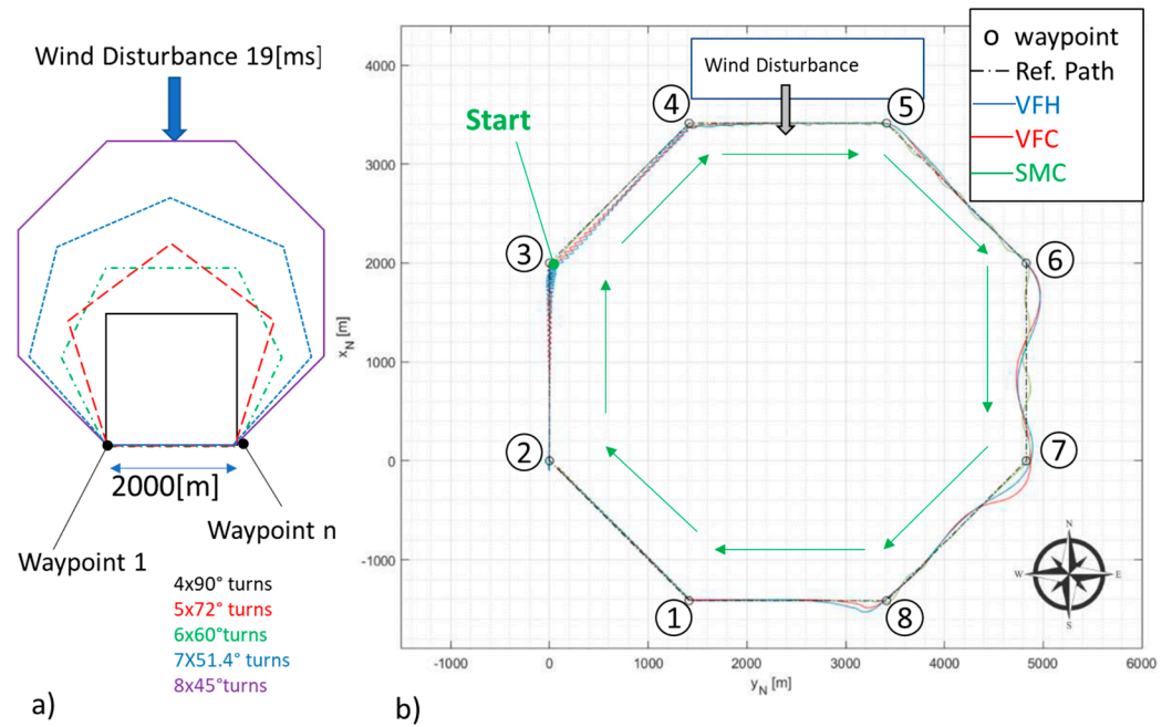
Figure 11. Different closed paths with polygonal shape (a), example of simulation performed with an octagonal one (b).
