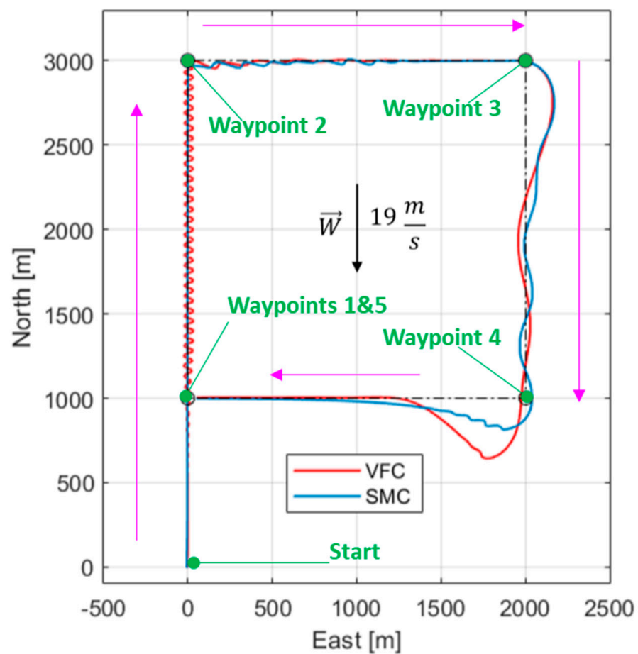
Figure 10. Comparison of course-based control algorithms in a high-wind scenario.
