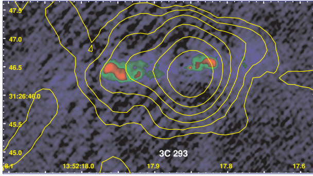
Figure 6. 3C 293. A 4.86 GHz radio image from a MERLIN observation which shows the brighter, inner radio structure. The X-ray contours come from a rebinned image as in Figure 1. The smoothing function is a Gaussian of FWHM = 0''.6 . Contours begin at 0.05 \text{ counts pixel}^{-1} and increase by factors of 2. (Radio map available on the Merlin archive.)
