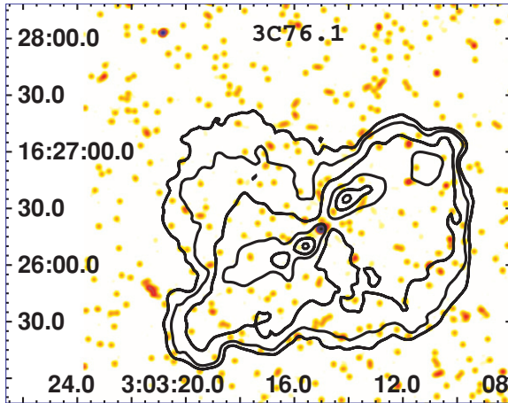
Figure 14. 3C 76.1. Flux map: f2; FWHM = 6'1.5 GHz radio contours start at 1 \text{ mJy beam}^{-1} and increase by a factor of 2. (Radio map available on the website: http://www.jb.man.ac.uk/ , "An Atlas of DRAGNs".)
