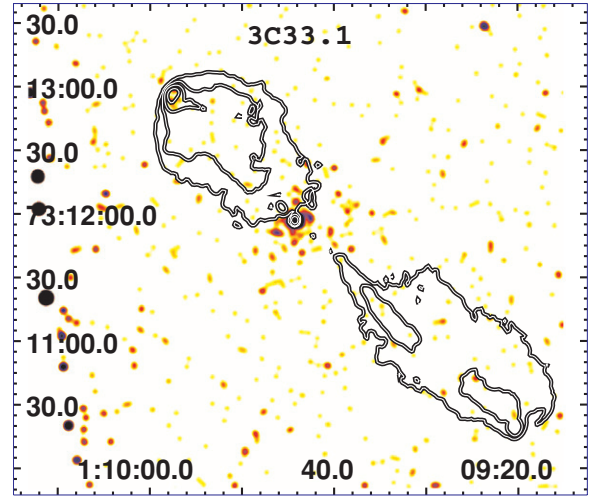
Figure 11. 3C 33.1. Flux maps: f2; FWHM = 6′.3. Radio (4.85 GHz) contours: 0.25 mJy beam −1 , increasing by a factor of 4. (Radio map kindly supplied by M. Hardcastle.)
