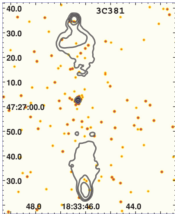
Figure 35. 3C 381. Flux map: f4; FWHM = 0''.5 . 8.44 GHz radio contours: 1 \text{ mJy beam}^{-1} , increasing by factors of 4. (Radio map kindly supplied by M. Hardcastle.)
