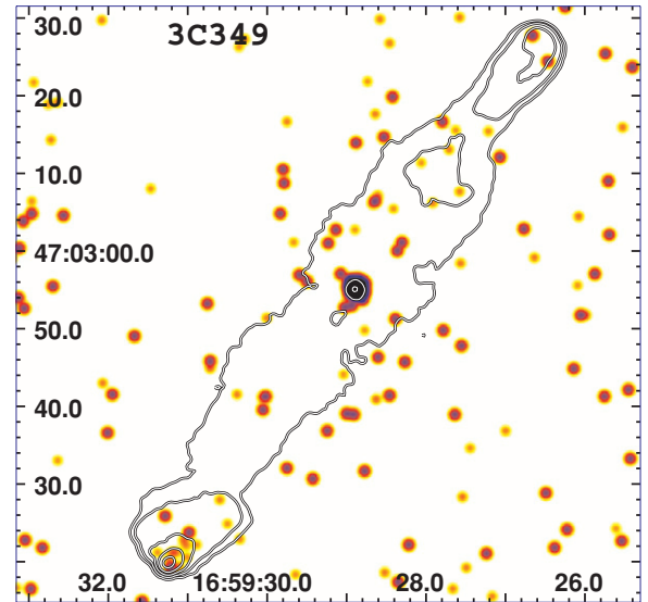
Figure 34. 3C 349. Flux map: f4; FWHM = 1''.5 GHz radio contours: 1 \text{ mJy beam}^{-1} , increasing by factors of 4. (Radio map available on the website: http://www.jb.man.ac.uk/ , “An Atlas of DRAGNs”.)
