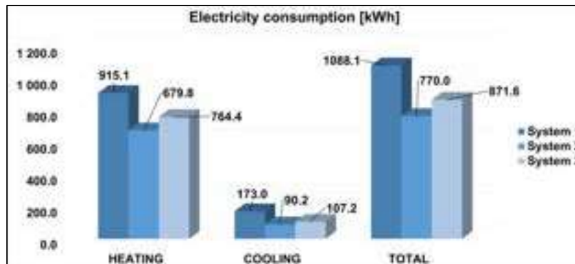
Figure 7. Comparison of electricity consumption for the different systems.
