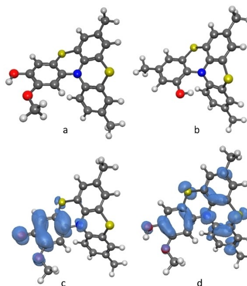
Figure 5. Optimized structures and spin densities of 8 (a), 7 (b), phenoxyl radical \text{8(-H)}^\bullet (c) and radical cation \text{8}^{\bullet+} (d).
