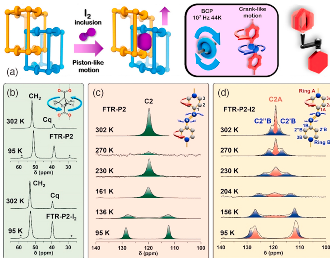
Fig. 12. Stimuli-responsive dynamics in a flexible pillared MOF. (a) Rotational motion of bicyclopentane (BCP), bipyridyl, and azopyridine (Azy) units is triggered by external stimuli such as I_2 vapors and pressurized CO_2 , enabling molecular-level motion within a pillared framework. (b–d) Variable-temperature ^{13}C CP MAS NMR spectra highlighting local dynamics: (b) BCP CH_2 and quaternary carbon signals in FTR-P2 (top) and FTR-P2- I_2 (bottom); (c) Azy C2 signal in FTR-P2; (d) Azy C2 signal in FTR-P2- I_2 . Adapted with permission from Ref. [58]. © 2024 Wiley-VCH GmbH.
