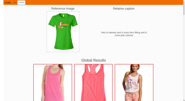
Figure 8. Results demo page. The user can check the results of the multimodal query he has inserted. Furthermore, by clicking on a retrieved image they can use it as reference image in a new query
