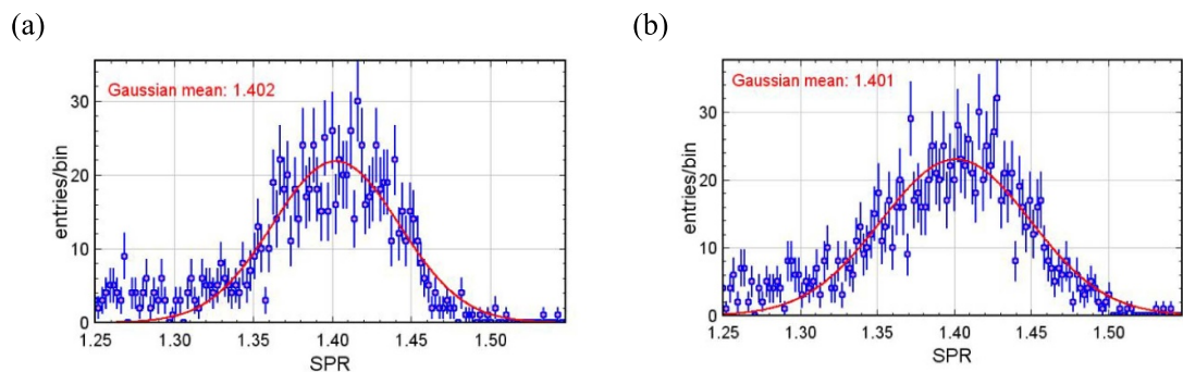
Figure 5. SPR distribution of the voxels inside 3D ROIs of phantom #2 identifying (a) the carbon rod #1a and (b) carbon screw #1b. The curve superimposed is a fit with a Gaussian function.
