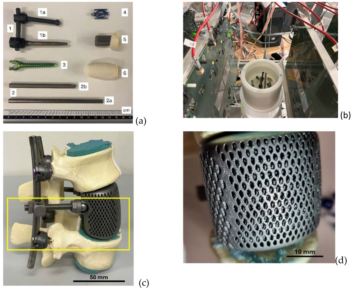
Figure 2. (a) Implant devices inspected by the pCT system: their description is reported in table 1. (b) Phantom #2 with the prosthesis' devices installed in the pCT system. (c) Photograph of the intra-vertebral titanium implant used for phantom #3 ; the yellow rectangle indicates the field-of-view of the tomographic image shown in this paper. (d) Detail of the Ti-alloy lattice structure.
