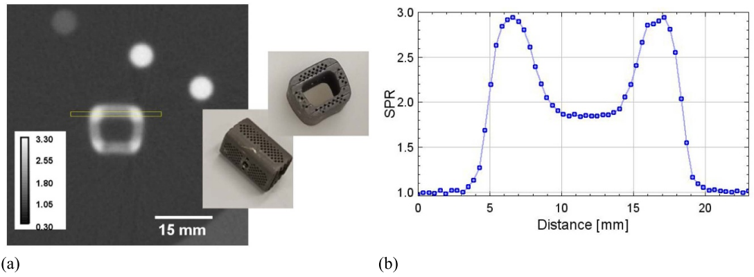
Figure 7. (a) zoom of axial slice in the correspondence of device #5 pictured in insets. (b) SPR profile along the ROI shown in yellow in (a).
