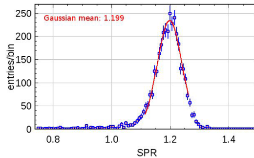
Figure 9. Distribution of the SPR in ROI2 (see text) within the cement material; the distribution is fitted using a Gaussian in a region of SPR between 1.1 and 1.3.
