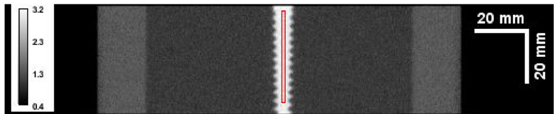
Figure 8. Coronal view of the self-tapping screw #3, showing the 3 mm pitch screw threads. Reconstruction voxel size of this image is 390\ \mu\text{m} \times 390\ \mu\text{m} \times 390\ \mu\text{m} . The ROI used to measure the material SPR is highlighted in red.
