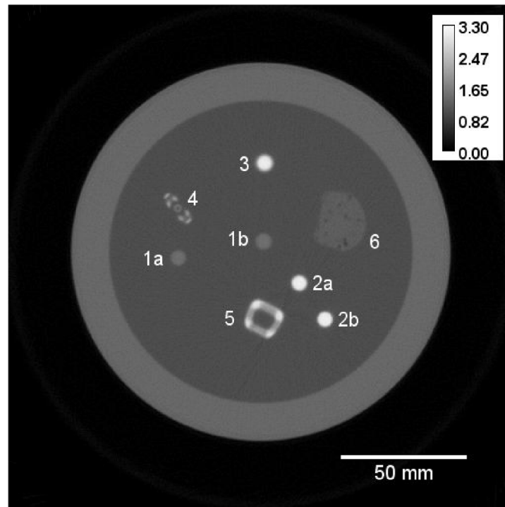
Figure 4. An axial slice of the prosthesis material and device phantom ( phantom #2 ). Labels identify the devices described in table 1. Gray scale indicates the SPR values.
