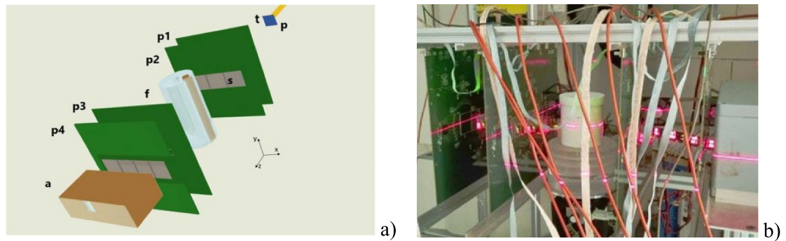
Figure 1. (a) Sketch of the pCT system: a: YAG:Ce calorimeter, p1 – p4 : tracker planes, s : silicon microstrip sensors, f : phantom, p : beam pipe; t : tantalum scattering plate (distance from tracker not to scale). The overlap sensor regions are visible in darker grey in the silicon microstrip sensors windows. Reproduced from Scaringella et al 2023. The Author(s). CC BY 4.0. (b) Photograph of the pCT system at the experimental beam line of Trento Proton Therapy Centre APSS, Trento, Italy.
