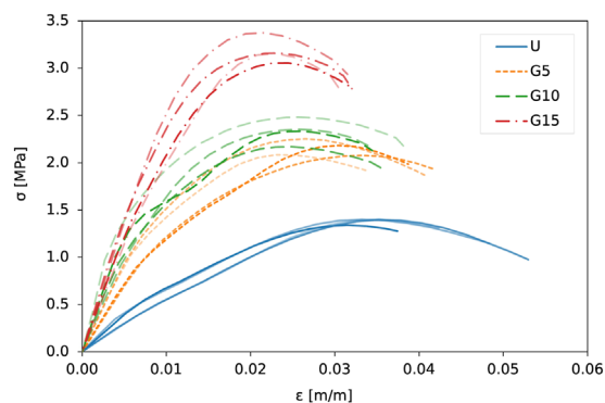
FIGURE 4 Stress-strain curves of the rammed earth samples obtained from uniaxial compression tests.
