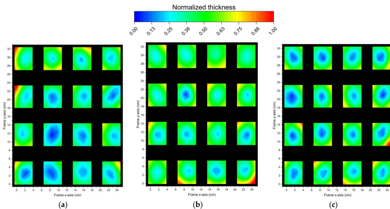
Figure 5. Normalized distributions of electrodeposited gold thicknesses, measured by XRF analysis, relative to a sample obtained (a) under standard conditions (DC1); (b) using the RAEP system; (c) using the HCS. The x and y axes represent the coordinates inside the plating rack, which contains 16 plates arranged in rows and columns of 4. Areas of the rack where there are no plates are shown in black.
