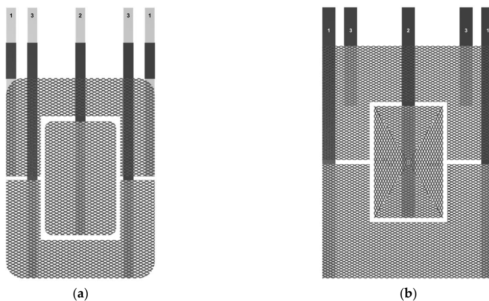
Figure 4. Anode schemes of (a) the Italfimet RAEP system, where 1 indicates the connectors related to the upper section of the three-anode system, 2 the connector related to the middle section and 3 the connector related to the lower section; (b) the LBT HCS system, where 1 indicates the connectors related to the lower section of the three-anode system, 2 the connector related to the middle section and 3 the connector related to the upper section.
