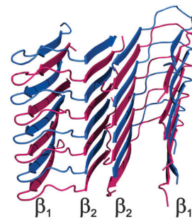
Fig. 3 Structural model of \text{A}\beta(1-40)/\text{A}\beta(1-42) interlaced mixed fibrils. The \text{A}\beta(1-42) polypeptide is colored in magenta while the \text{A}\beta(1-40) polypeptide in blue.
