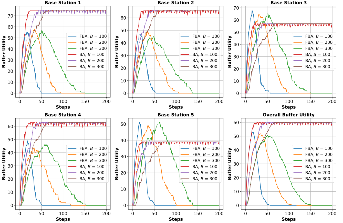
Fig. 11. Buffer utility for different values of buffer length versus steps.
