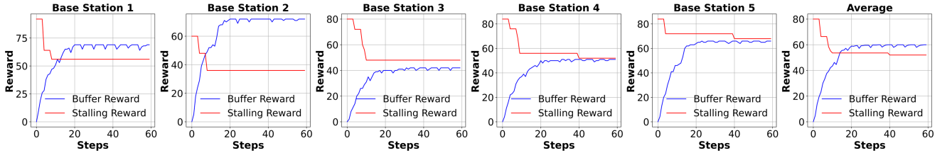
Fig. 12. Buffer and stalling rewards versus steps.
