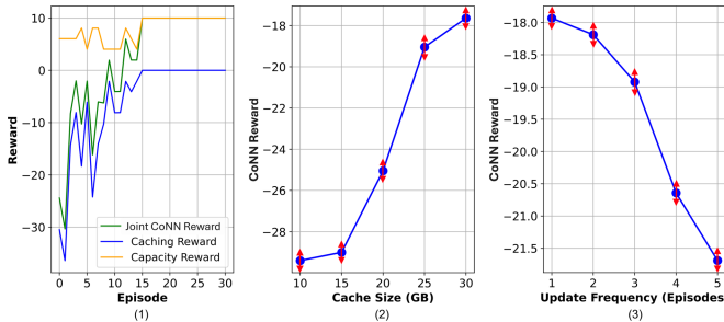
Fig. 8. (a) Caching, capacity and joint CoNN rewards versus episodes, (b) CoNN reward vs cache size, and (c) CoNN reward vs update frequency.
