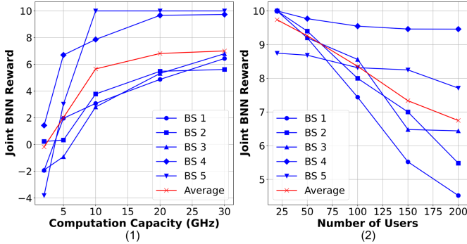
Fig. 10. Joint BNN reward versus: (a) Computation capacity, and (b) number of users.
