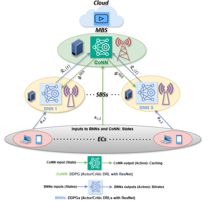
Fig. 6. Overall architecture of CoNN-BNNs-environment interactions.
