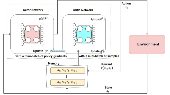
Fig. 5. DDPG-based DRL actor/critic architecture.
