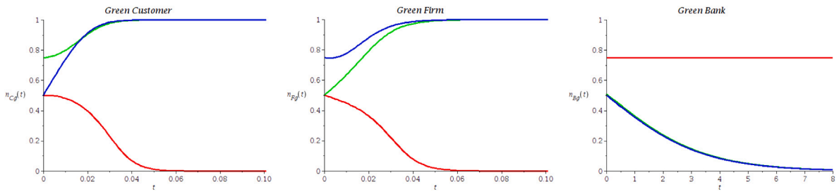
Fig. 5. The time series of n_{C_g} , n_{F_g} , and n_{B_g} in Simulation V, with initial conditions of 50% or more of customers, firms, and banks choosing green sustainability. (For interpretation of the references to color in this figure legend, the reader is referred to the web version of this article.)
