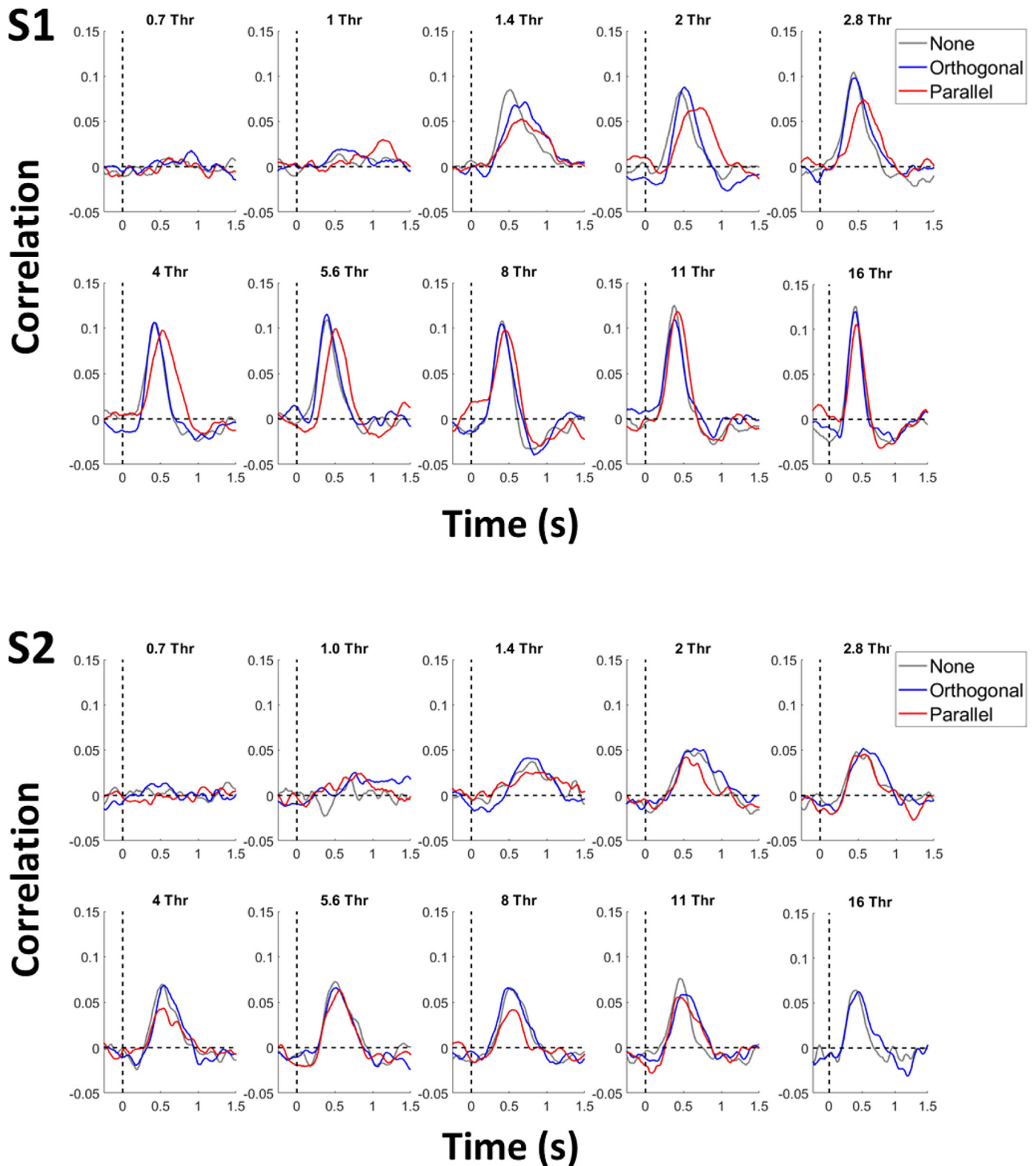
Figure 3. Results of the first tracking experiment on two of the four participants. Gray, blue, and red curves are the cross-correlations between target movements and mouse movements in the presence of the nonoriented, orthogonal, and parallel masks, respectively. In each panel, target contrast is a fixed multiple of each participant's detection threshold for each mask, shown at the top of each panel.
