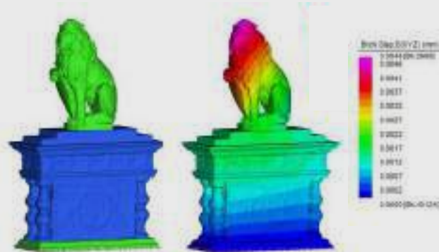
Fig. B FEM (FiniteElement Method) applied on the 3D model of Donatello's Marzocco: static analysis for vertical loads
