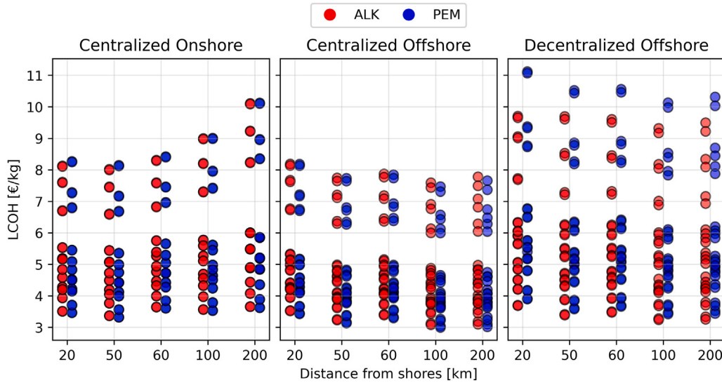
Fig. 13. Range of LCOH for each system configuration for five wind park sites, characterized by their distance to shore.
