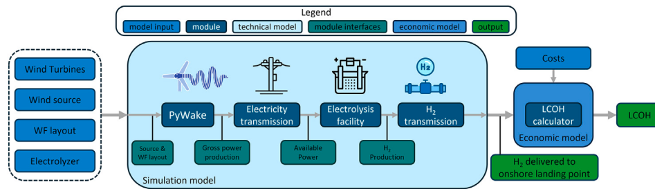
Fig. 1. Simulation model workflow.
