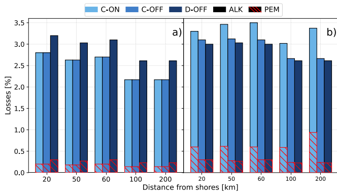
Fig. 14. Overview of the operational behavior of the offshore configurations with PEM and ALK with the inclusion of additional wind park sites HKZ (20 km) and LJV (60 km).
