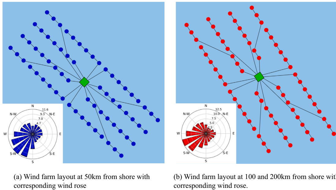
Fig. 3. The dots represent the wind turbines, and the lines represent the IA cables (centralized system configurations) or pipelines (decentralized system configuration). The green square in the middle represents the centralized substation for electrical or hydrogen transmission to shore.
