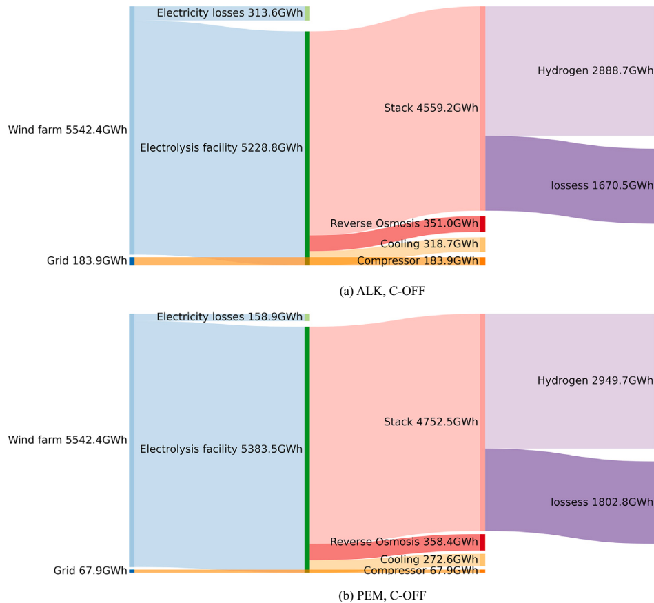
Fig. 10. Sankey diagrams for the ALK and PEM electrolyzers in the C-OFF system configuration.
