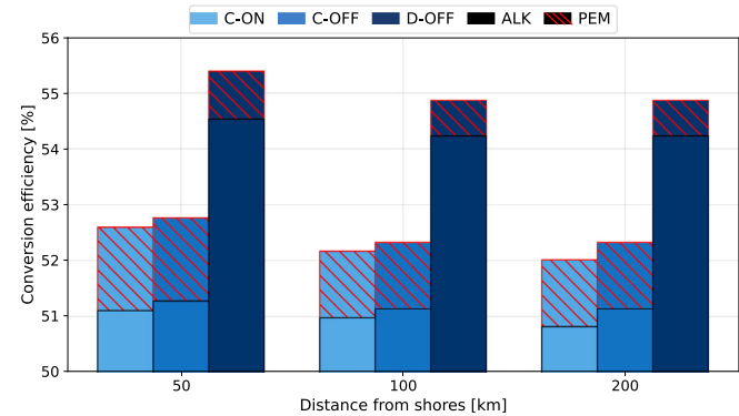
Fig. 8. Mean overall system efficiency across all scenarios and configurations.
