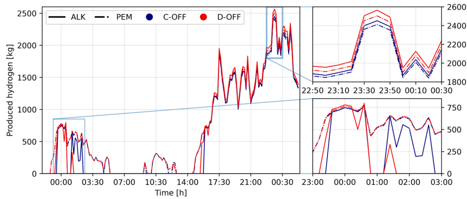
Fig. 12. Comparison between the operational behavior of the offshore configurations with PEM and ALK.
