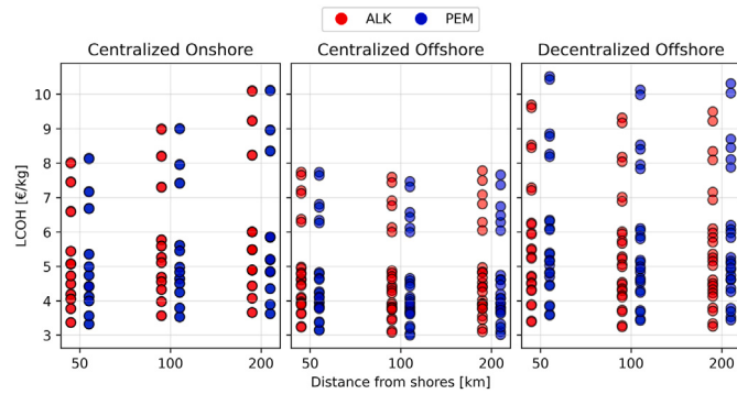
Fig. 5. Range of LCOH found for each system configuration for three wind park sites (characterized by their distance to shore).
