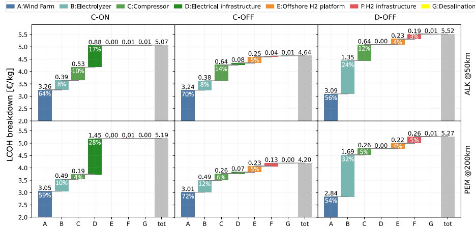
Fig. 6. LCOH breakdown for two scenarios (under expert validated cost and mean technology input data) for each system configuration: a 50 km offshore distance using an ALK electrolyzer, and a 200 km offshore distance using a PEM electrolyzer.
