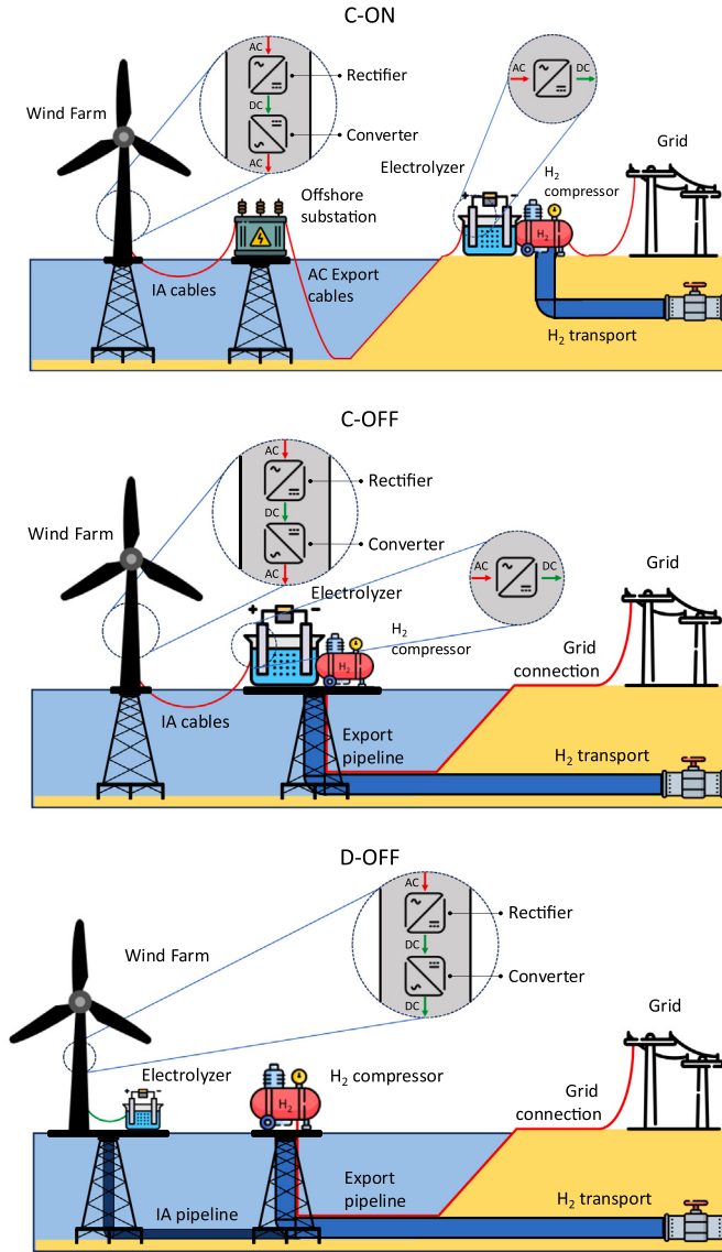
Fig. 4. Schematic representation of the C-ON, C-OFF and D-OFF system configuration.
