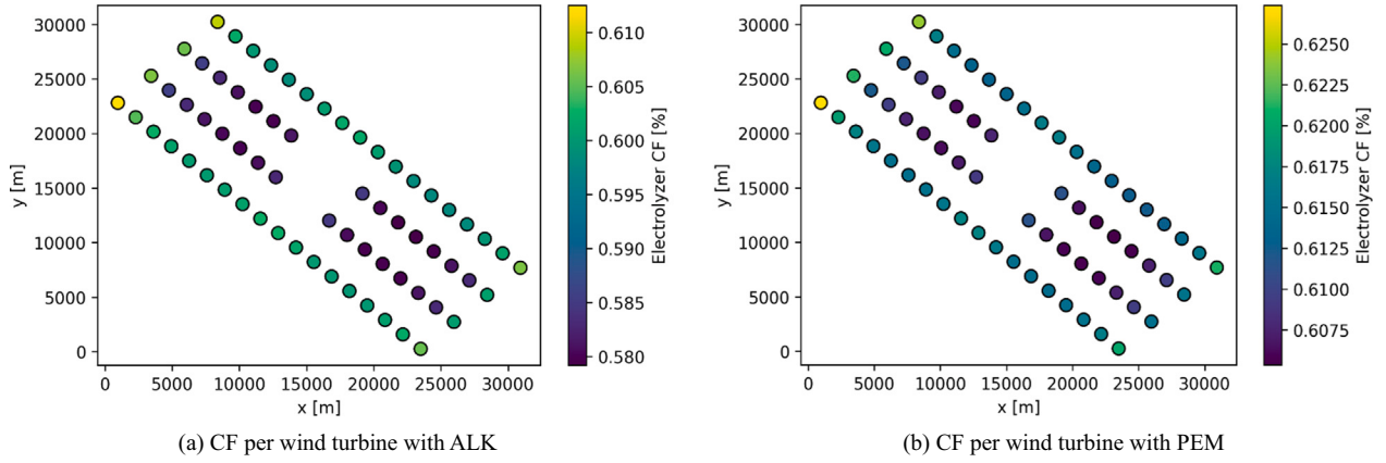
Fig. 11. Capacity factor (CF) per wind turbine in the D-OFF configuration for the mean technical scenario in the 100 km offshore site.
