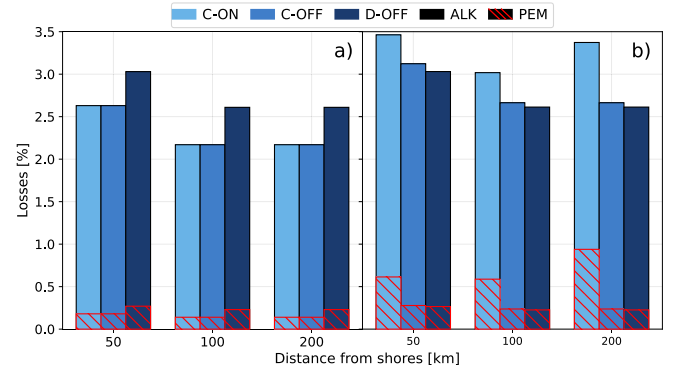
Fig. 9. Losses due to electrolyzer constraints (a) (minimum load requirements, cold startups, and power electronics) and total losses (b) (including distance from shores) per system configuration.
