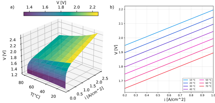
Fig. 2. Polarization curve of the PEM electrolyzer (a) [36] and ALK electrolyzer (b) [14].
