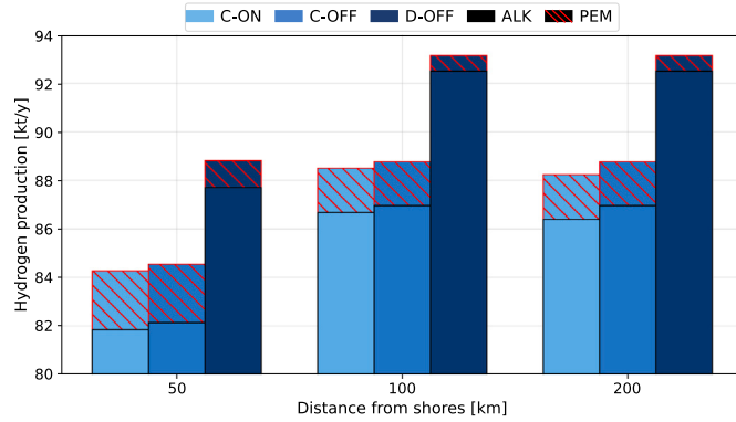
Fig. 7. Annual hydrogen delivered to the backbone for C-ON, C-OFF, and D-OFF for different distances to shores and electrolysis technologies in the mean technical scenario.
