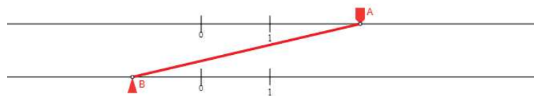
Dynagraph 4: f(x)=\text{round}(x)
