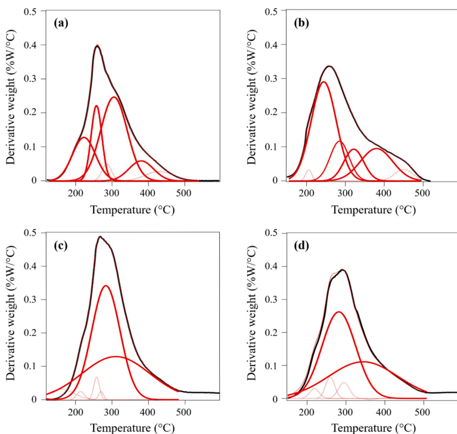
Fig. 1. Derivative thermogravimetric (DTG) curves (black lines) and corresponding deconvoluted signals (red lines) for EPS / sEPS from NaOH-based extraction (a / c) and for EPS / sEPS from \text{Na}_2\text{CO}_3 -based extraction (b / d). The red solid / dashed lines refer to the Gaussian contributions whose area is higher / lower than 5 % of the total area subtended by the DTG curve, respectively. The latter (dashed lines) are therefore marginal contributions that were not considered in the discussion.
