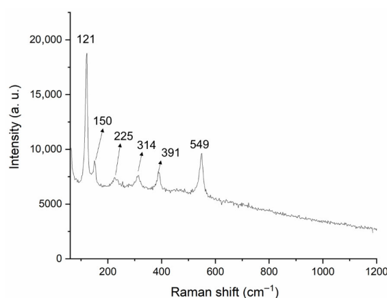
Figure 9. Raman spectrum of orange hue.
