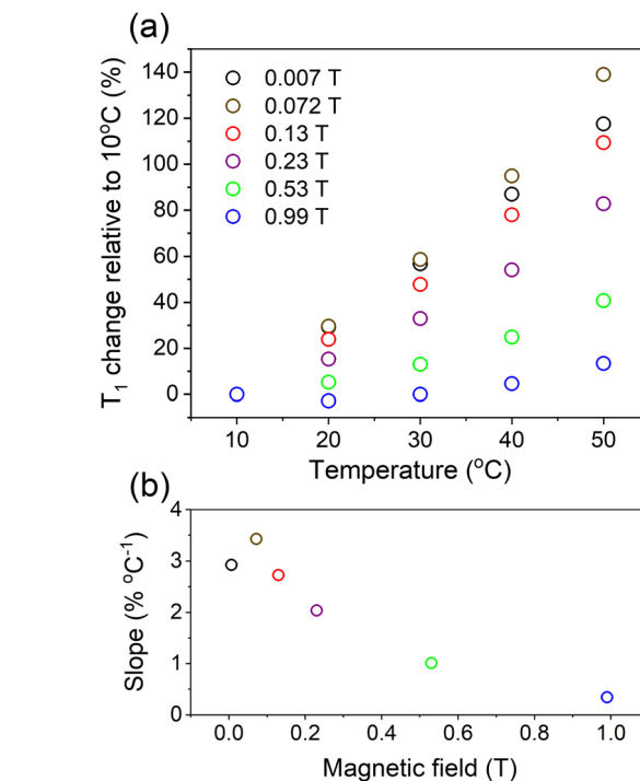
Fig. 5 Temperature and magnetic field dependence of T_1 for water hydrogen protons in agar gel with embedded MnZn iron oxide in concentration of 1.45 mM. (a) Percentage changes of T_1 . At various (b) value of the slopes from Fig. 5(a) normalized to 10–50 °C temperature range.
