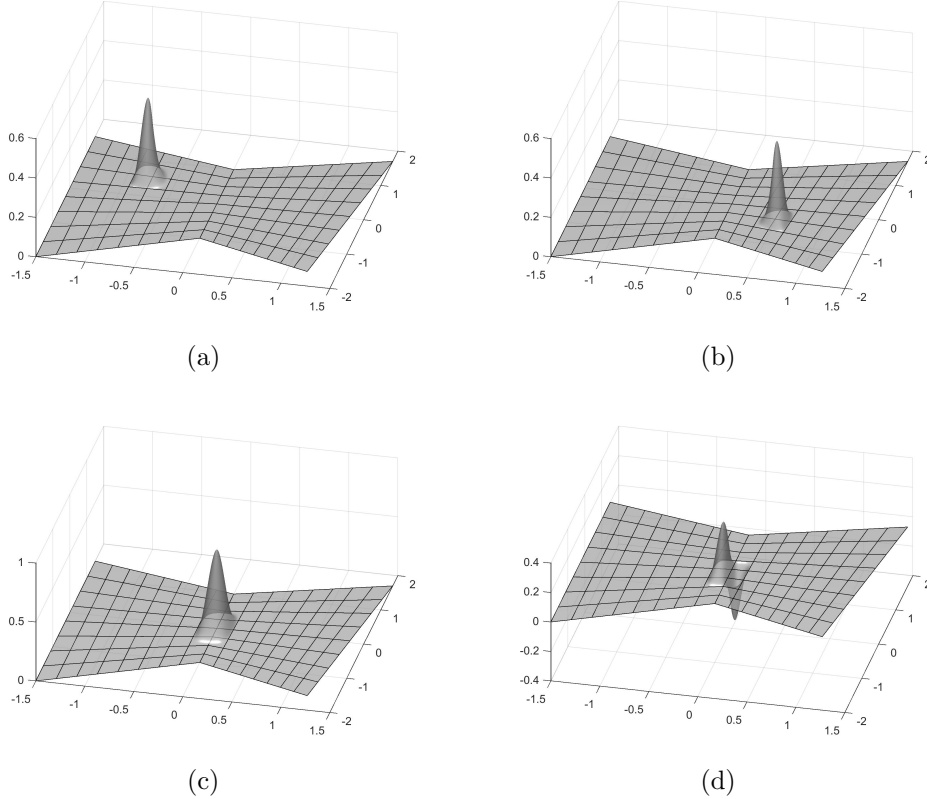
Figure 1: Example of basis functions of \mathbb{W} on a two-patch domain: figures (a)-(b) show two basis functions of type (13) (standard B-splines whose support is included in one of the two patches), while figures (c) and (d) correspond to basis functions of type (14) and (15), respectively (whose supports intersect the interface).
