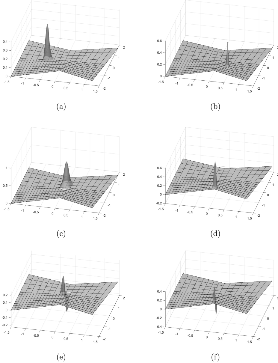
Figure 2: Example of basis functions of \mathbb{W}_H on a two-patch domain: on the left basis functions of type (13), (14) and (15) respectively belonging to level 0 are shown, while on the right analogous basis functions of level 1 are reported.
