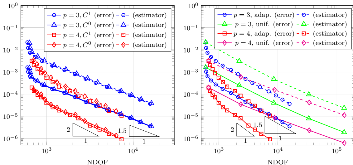
Figure 6: Relative error in H^1 semi-norm and corresponding estimator for Example 2 with \mathbf{p} = (3, 3) and \mathbf{p} = (4, 4) , compared with C^0 case (left) and with global refinement case (right).
