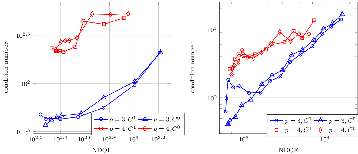
Figure 10: Comparison of the condition number of the stiffness matrix, after diagonal preconditioning, obtained in the solution of Example 1 (left) and Example 2 (right).
