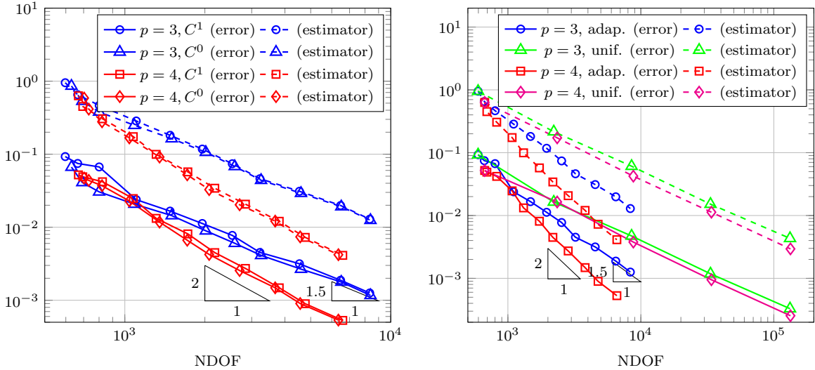
Figure 8: Error in H^1 semi-norm and estimator for Example 3 with \mathbf{p} = (3, 3) and \mathbf{p} = (4, 4) , compared with C^0 case (left) and with global refinement case (right).
