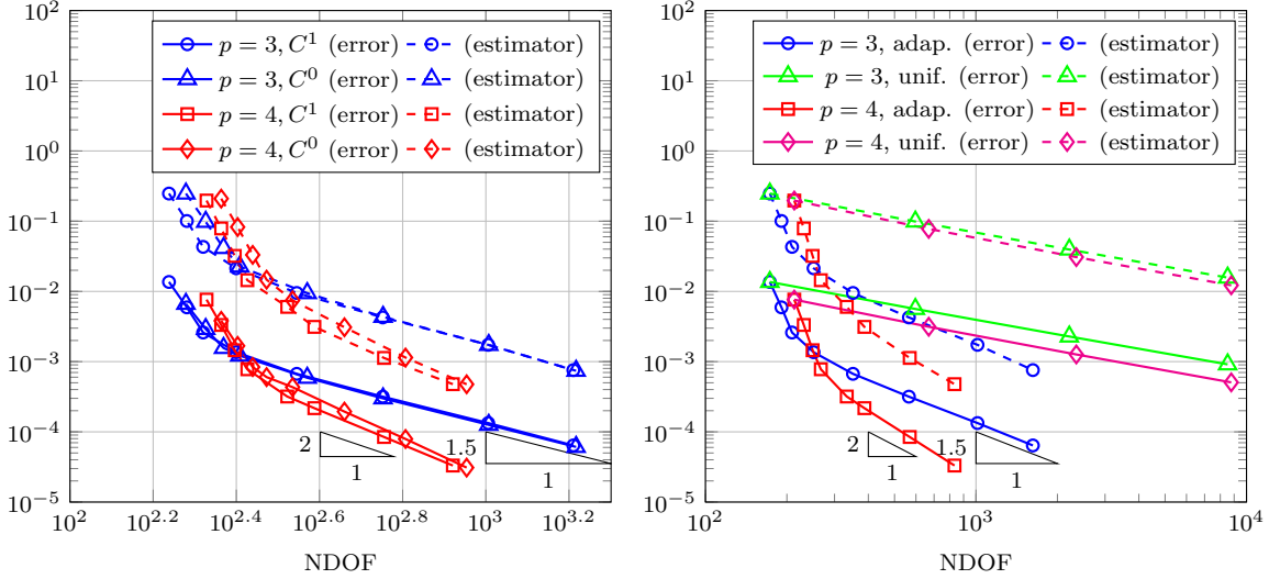
Figure 4: Error in H^1 semi-norm and estimator for Example 1 with \mathbf{p} = (3, 3) and \mathbf{p} = (4, 4) , compared with C^0 case (left) and with global refinement case (right).
