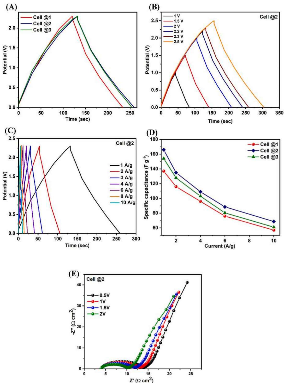
Fig. 7. (A) Comparative GCD curves for all the cells in the optimum voltage range 0–2.3 V and, (B) GCD curves of Cell @2 with varying voltage ranges recorded at current density 1 A g -1 , (C) GCD curves measured at different current densities from 1 to 10 A g -1 for Cell @2, (D) specific capacitance ( C_{sp} ) versus current density plot for all the EDLC cells, (E) impedance spectra of Cell @2 at different voltages.
