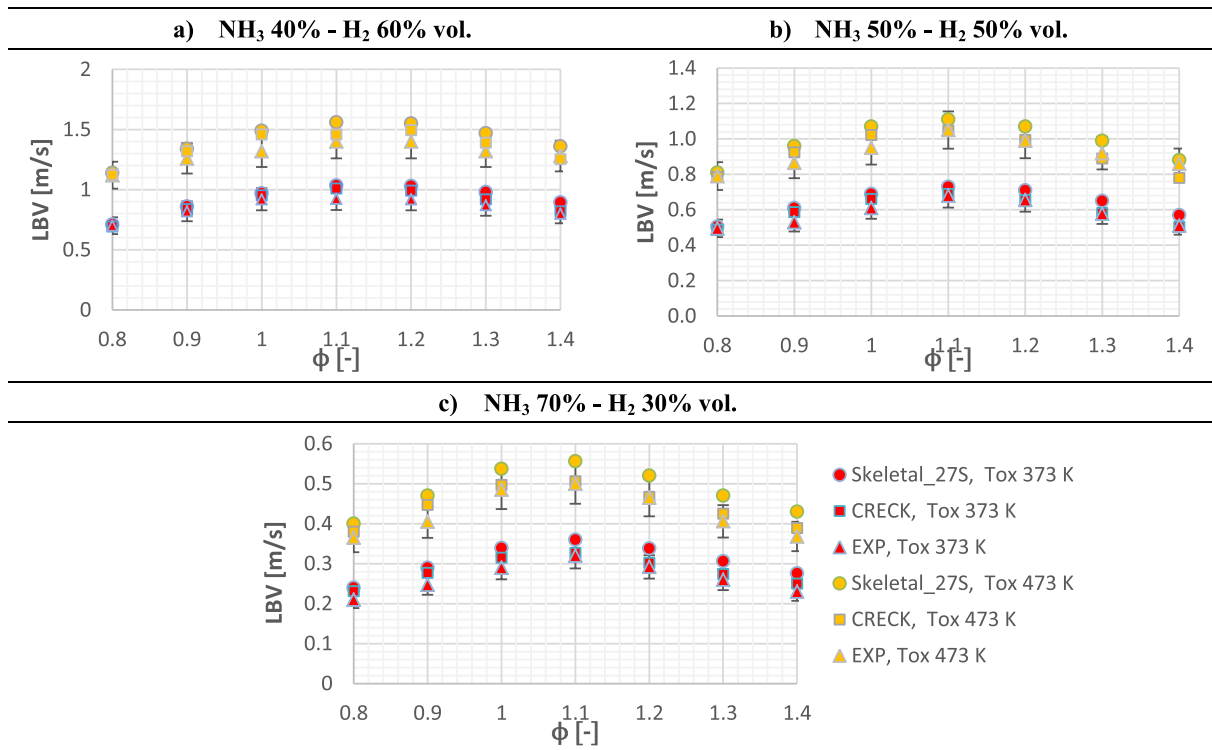
Fig. 6. LBV calculation with the skeletal and the original mechanism compared against the experimental measurements by Lhuillier et al. [35]. Data are collected at atmospheric pressure and two preheated air temperatures across the stoichiometric equivalence ratio. Three ammonia contents in the fuel are investigated: 40% (a), 50% (b) and 70% (c) by volume.
