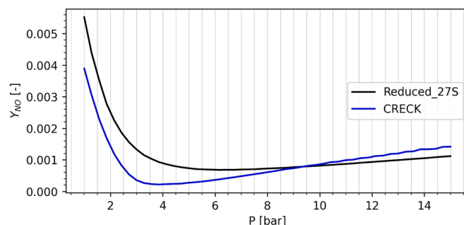
Fig. 8. NO emissions comparison between the detailed mechanism (CRECK) and the reduced mechanism. Results extracted from a PSR + PFR reactor network reproducing the overall combustion chamber residence time. The comparison refers to the operating conditions reported in Table 1.
