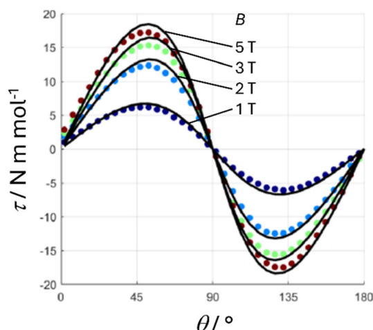
Fig. 6 Angular dependence of the magnetic torque of 1Fe measured at B = 1, 2, 3 , and 5 T (from indigo to wine) at T = 2 K. At the beginning of the clockwise rotation around the crystallographic a axis, the magnetic field was along the c crystallographic axis.
