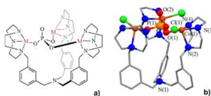
Figure 49. Drawing of ligand L54 (a) and crystal structure of the [CuCl_3(\mu_3-HPO_4)L54]^+ cation (b).
