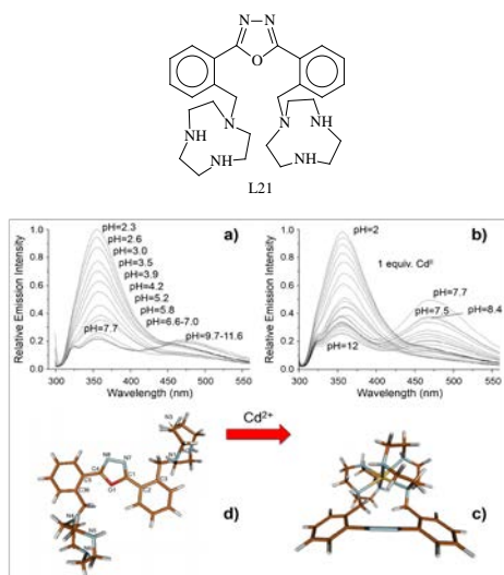
Figure 18. Fluorescence emission spectra in H 2 O of a) L21, and b) L21/Cd 2+ 1:1 molar ratio on changing the pH ([L21] = 2 × 10 -5 M, λ exc = 272 nm); DFT optimized geometries of c) [Cd(L21)]^{2+} (29), and d) L21. Adapted from Ref. [43] with permission from The Royal Society of Chemistry.
