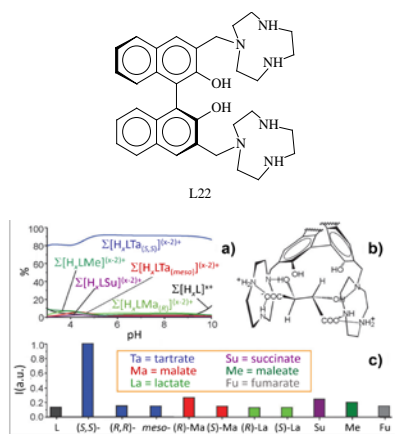
Figure 19. a) Plots of the overall percentages of the L22 complexed species with (S,S)-tartaric ( H_2Ta_{(S,S)} ), (R)-malic ( H_2Ma_{(R)} ), maleic ( H_2Me ) and succinic ( H_2Su ) acids on changing the pH in H 2 O, in a competitive system containing L22 and the acids in equimolar ratio (10 -3 M). b) proposed interaction mode of (S,S)-tartarate with (H_2L22)^{2+} ; c) normalized intensity emission at 410 nm (λ exc = 279 nm) after the addition of each substrate (10 equivs.) to a water solution of L22 at pH = 7.00. Adapted from Ref. [44] with permission from The Royal Society of Chemistry.
