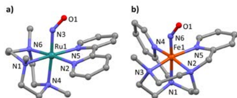
Figure 72. Ball and stick views of complexes 53 (a) and 54 (b). Hydrogens and counterions have been omitted for clarity. Fe orange, Ru petroleum green, O red, N blue, C gray. Figure 72a is adapted with permission from Ref. 177, Copyright © 2016, American Chemical Society. Figure 72b is reproduced from Ref. [178] with permission from The Royal Society of Chemistry.
