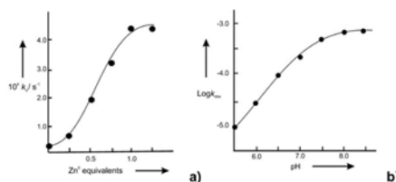
Figure 53. Dependence of the rate constant for the cleavage of HPNP by AuNP1-TACN on the amount of \text{Zn}^{2+} ions ( 40^\circ\text{C} , pH 7.5, [\text{AuNP1-TACN}] = 0.1 \text{ mM} ) (a) and of the rate of cleavage of HPNP by \text{Zn}^{2+} -AuNP1-TACN as a function of pH ( 40^\circ\text{C} , [\text{Zn}^{2+}\text{-AuNP1-TACN}] = 0.1 \text{ mM} ). Adapted from Ref. [122] with permission from John Wiley and Sons. Copyright © 2004.
