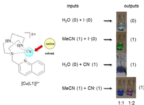
Figure 3. Truth table of the OR operation performed by [\text{Cu}(\text{L1})]^{2+} on solvents [ \text{H}_2\text{O} (0), MeCN (1)] and anions [ \text{I}^- (0), \text{CN}^- (1)] inputs. In the case of MeCN as solvent and \text{CN}^- as anion, two distinct colours can be observed depending on the 1/ \text{CN}^- molar ratio. Reprinted from Ref. [18] with permission from Elsevier. Copyright © 2014.
