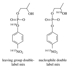
Figure 47. Sketch of the isotopically marked HPNP substrates used to elucidate the cleavage mechanism catalyzed by 43
