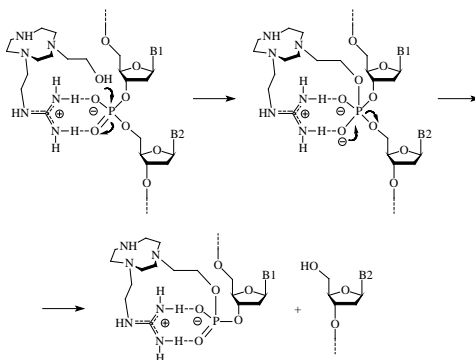
Figure 38. Proposed mechanism for DNA cleavage by L43. A similar mechanism, involving possible Zn 2+ -assisted deprotonation of the ethanolic pendant followed by the nucleophilic attack of the R-O-generated function is also suggested its Zn 2+ complex 41 .
