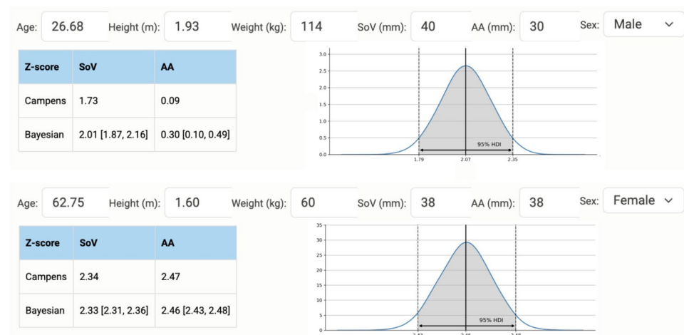
Fig. 2. Conditional densities for the Bayesian Z-score. Top: SoV for a 26-year-old male patient with 1.93m height, 114 kg weight, and 40 mm SoV diameter; the expected Z in this case is near 2 but the density is not concentrated and its interval is large, i.e., there is a significant probability that Z is actually above or below 2. Bottom: AA for a 62-year-old female patient with 1.60m height, 60 kg weight, and 38 mm AA diameter; in this case the density is concentrated and the whole interval is well above 2. Therefore, the patient can be safely assumed to be dilated. Both patients in these examples were diagnosed with Marfan syndrome. Note that conditional densities of Z are not Gaussian and thus not necessarily symmetric around the mean.
