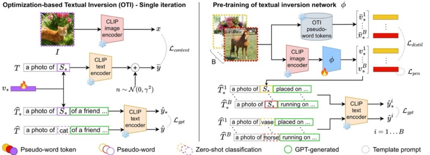
Fig. 2. Overview of our approach. Left : single iteration of the iterative Optimization-based Textual Inversion (OTI) method to generate a pseudo-word token v_* from an image I . We force v_* to represent the image content with a cosine loss \mathcal{L}_{content} . We add Gaussian noise to the text features before computing \mathcal{L}_{content} . We assign a concept word to I with a CLIP zero-shot classification and feed the prompt “a photo of {concept}” to GPT to continue the phrase, resulting in \hat{T} . Let S_* be the pseudo-word associated with v_* . We craft \hat{T}_* by replacing in \hat{T} the concept with S_* . \hat{T}_* and \hat{T} are then employed for a contextualized regularization with \mathcal{L}_{gpt} . Right : pre-training of textual inversion network \phi on unlabeled images. Given a set of pseudo-word tokens pre-generated with OTI, we distill their knowledge to \phi through a contrastive loss \mathcal{L}_{distil} . We regularize the output of \phi with the same GPT-powered loss \mathcal{L}_{gpt} employed in OTI and an additional penalty term \mathcal{L}_{pen} . B represents the number of images in a batch.
