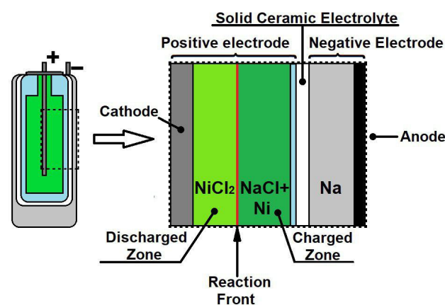
Figure 3. A schematic description of the SMHC during the discharge phase.
