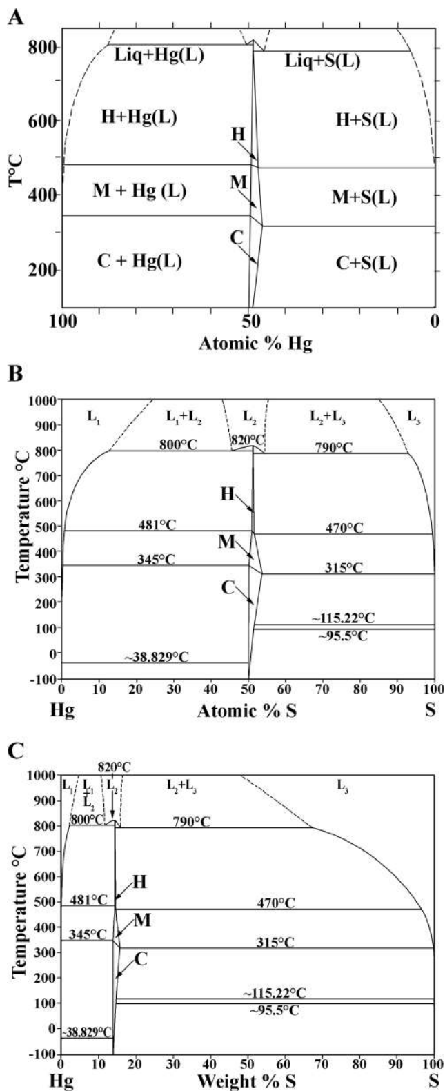
Fig. 4 Phase relations. A Modified from Potter and Barnes (1978); B–C simplified after Sharma et al. (1993) (C=cinnabar; M=metacinnabar; H=hypercinnabar)
