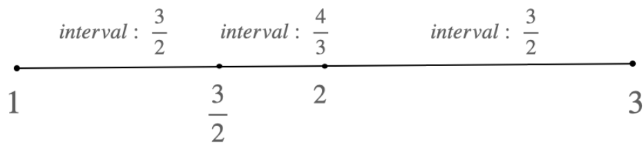
Figure 11. Harmonic and arithmetic mean: the two 3/2 intervals and the 4/3 interval in [1,3] .
