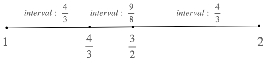
Figure 3. Harmonic and arithmetic mean: the two 4/3 intervals and the 9/8 interval.
