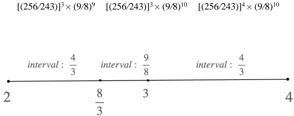
Figure 8. Harmonic and arithmetic mean: the two 4/3 intervals and the 9/8 interval in the interval [2,4].
