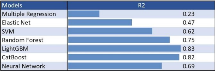
Figure 2 – R^2 of the different trained models.
