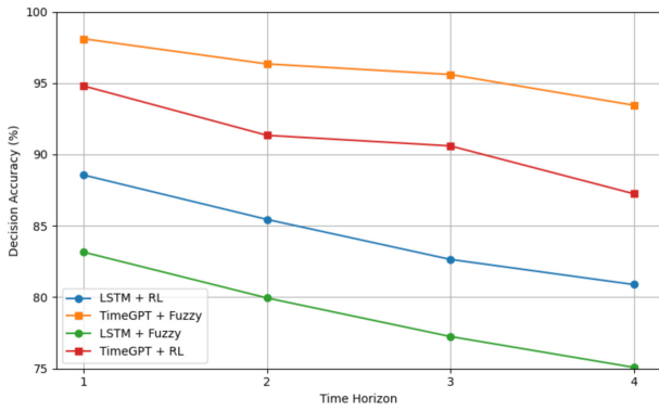
Fig. 7. Decision accuracy of the offloading process, comparing the LSTM + RL baseline with the proposed TimeGPT + Fuzzy Logic framework. The figure reports the accuracy of the decision-making process over different prediction horizons, highlighting the benefits of combining zero-shot forecasting with symbolic reasoning.
