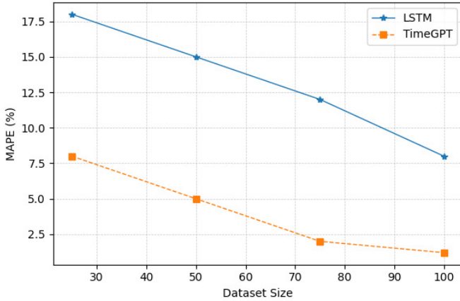
Fig. 8. MAPE as a function of the dataset size for LSTM and TimeGPT, i.e., as a function of the size window l .
