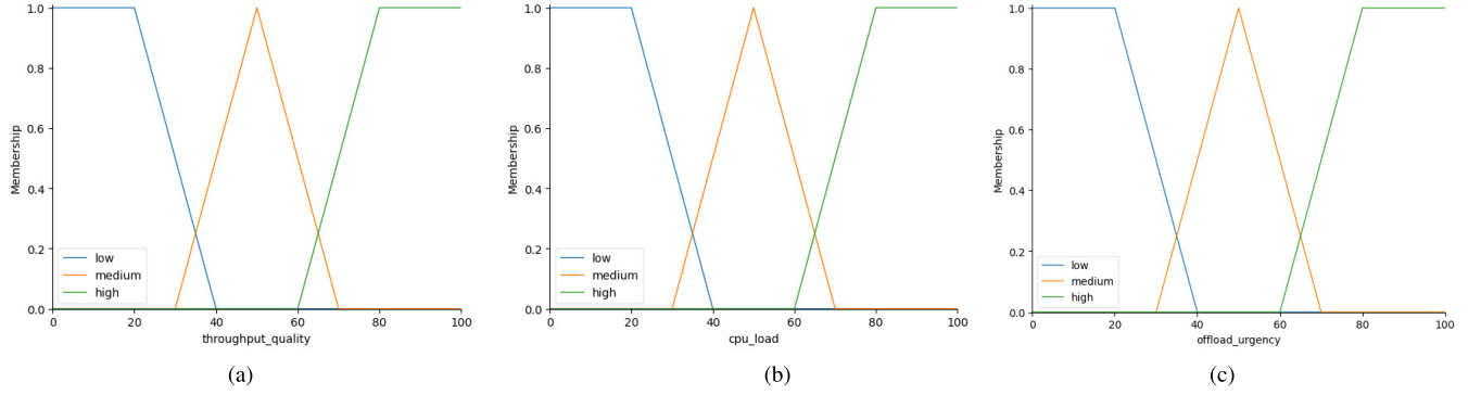
Fig. 6. Membership functions for the considered quality metrics, namely satellite link throughput quality, satellite CPU load, and offloading urgency, used by the FLC to translate continuous predictions into linguistic variables. (a) Membership function of throughput quality. (b) Membership function of CPU load. (c) Membership function of offloading urgency.
