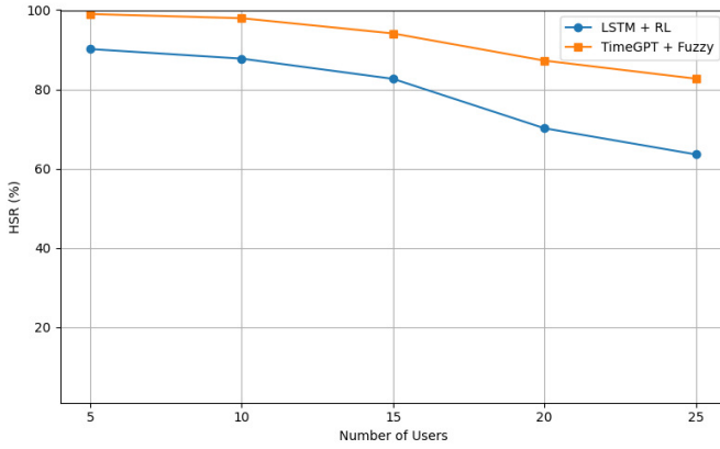
Fig. 9. HSR as a function of the number of users requesting offloading, assuming an average of ten satellites in line-of-sight. The figure compares the proposed TimeGPT + Fuzzy matching approach against the LSTM + RL baseline, showing that the proposed method consistently achieves higher user satisfaction and degrades more gracefully under increasing resource contention.
