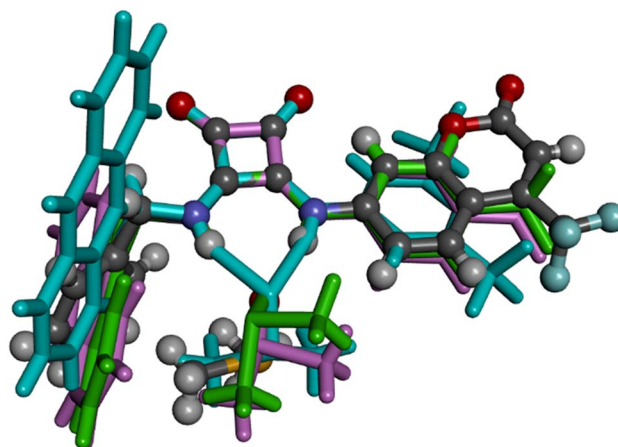
Fig. 4 Superimposition of L1·DMSO (ball and stick) with CIPYIL (stick, pale blue), CIPYOR (stick, pale green) and CIPYUX (stick, pale pink).
