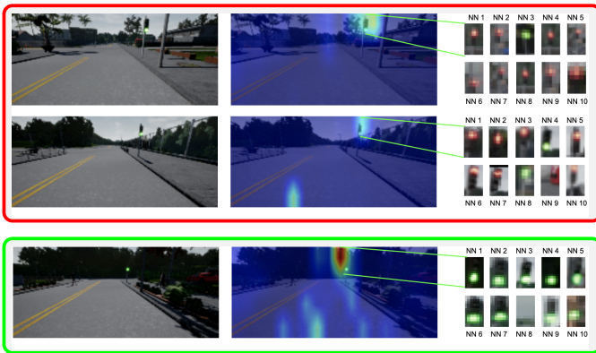
Fig. 4. Top 10 neighbors for the highest scoring attention after a traffic light turns green. We show examples of both successful crossing of the traffic light (framed in green) and failed due to red light "hallucination" (framed in red).
