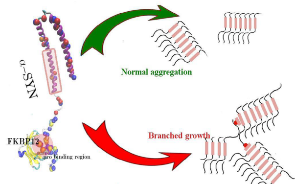
Figure 5 Mechanism for FKBP12-driven aggregation of \alpha -syn. On the left, a ribbon representation of \alpha -syn bound to FKBP12. The NAC domain in \alpha -syn is highlighted in light salmon color. In orange, we show the Try82 and Ile56 of the catalytic site of FKBP12 interacting with an \alpha -syn Pro at the C terminus. On the right, we show how, when bound to \alpha -syn hydrophilic C terminus, FKBP12 promotes branched fibrillar growth with beta stacking of the \alpha -syn NAC domains. \alpha -syn: \alpha -Synuclein.
