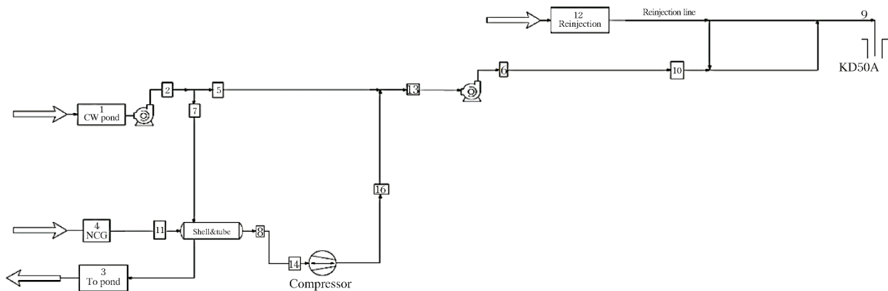
Fig. 2. NCG reinjection system.
