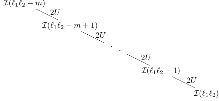
Figure 6: The graph \mathcal{G}_1 in both the subcritical and the supercritical case.
