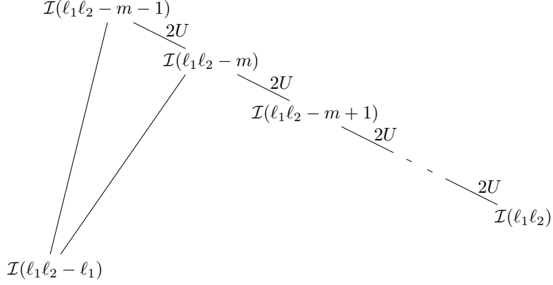
Figure 7: The graph \mathcal{G}_2 in the subcritical case.
