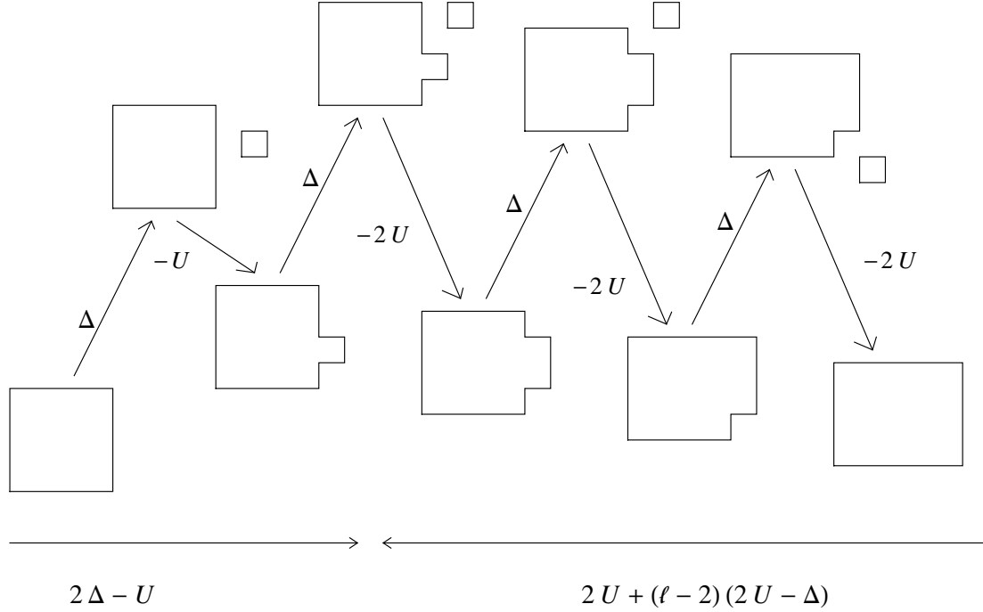
Figure 4: Cost of adding or removing a row of length \ell in a finite volume.
