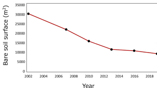
Fig. 7. Changes in the extent of bare soil surfaces from 2002 to 2019 in the Leonina biancana field. Data obtained by photo-interpretation of aerial orthophotos (Tuscany Region, 2022b), with a minimum mapping unit of 10 m 2 , in QGIS v. 3.20.3 (QGIS Development Team, 2021).
