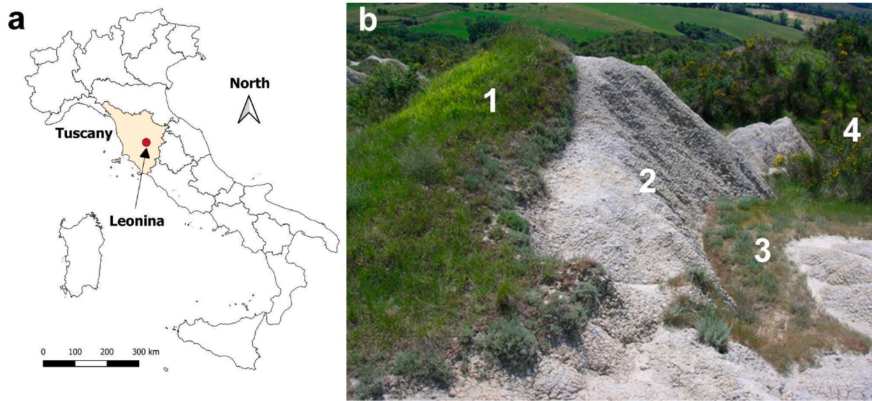
Fig. 1. a) Location of the study area in Italy and Tuscany; b) biancana in the Leonina field with different vegetation types developing on soils with different salinity and erosion rates: 1) upper part of a biancana with perennial Bromopsis erecta grassland; 2) bare soil with little or no vegetation on a southern biancana slope; 3) biancana pediment with Artemisia caerulescens subsp. cretacea and Parapholis spp. pioneer vegetation; 4) Spartium junceum shrubland.
