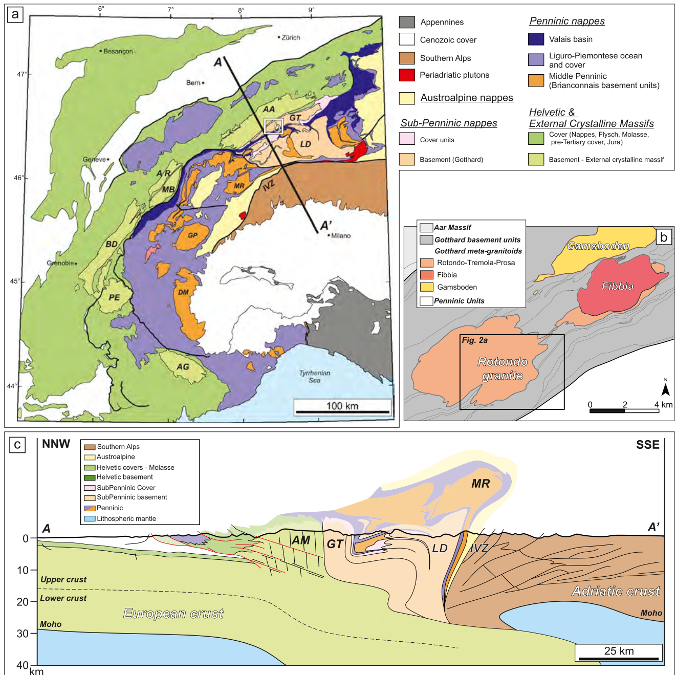
Figure 1. Geological setting of the study area. (a) Tectonic sketch of the Central-Western Alps (redrawn from Ballèvre et al., 2018, Schmid et al., 2004; Schwartz et al., 2024). AA: Aar; AG: Argentera; AR: Aiguilles rouges; BD: Belledonne; DM: Dora Maira; GP: Gran Paradiso; GT: Gotthard; IVZ: Ivrea-Verbano Zone; LD: Leptontine Dome; MB: Mont Blanc; MR: Monte Rosa; PE: Pelvoux. (b) Tectonic sketch of the Central-Western Gotthard massif showing the spatial distribution of the meta-granitoid intrusion (Rotondo, Fiabba, Gamsboden). (c) Geological section across the Central Swiss Alps.
