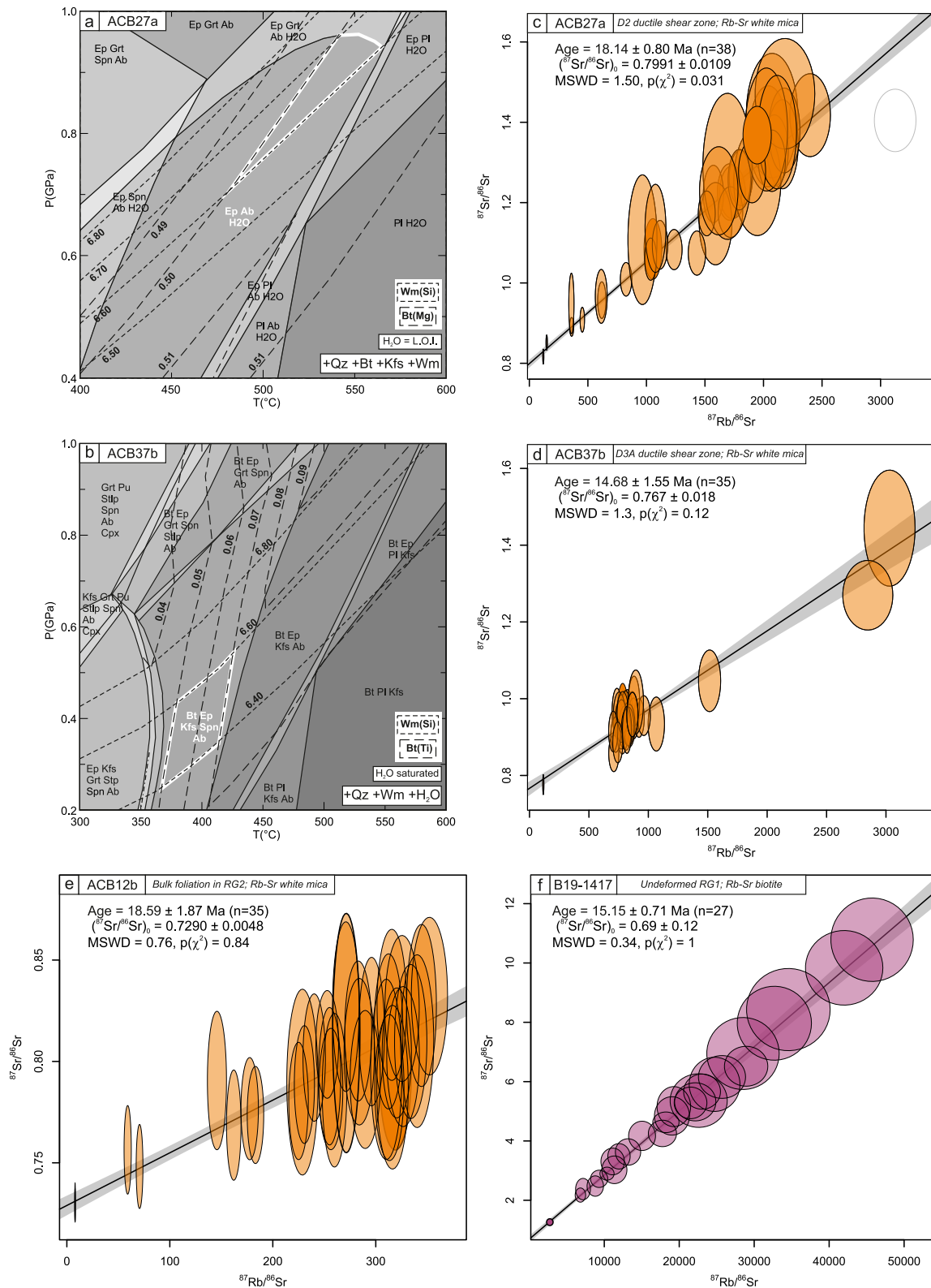
Figure 9. P-T-t data for sample ACB27a–ACB37b. (a–b) Computed pseudosections for sample ACB27a and ACB37b, respectively. (c) ACB27a, (d) ACB37b, (e) ACB12b, and (f) B19-1417 mica Rb–Sr isochrones including their corresponding ages (slope) and initial ^{87}\text{Sr}/^{86}\text{Sr} composition (intercept). The size of the ellipses indicates internal 2SE (standard error). Isochronous regressions are plotted as black lines with their 95% confidence level as gray envelopes. All plots were generated using IsoplotR (Vermeesch, 2018).
