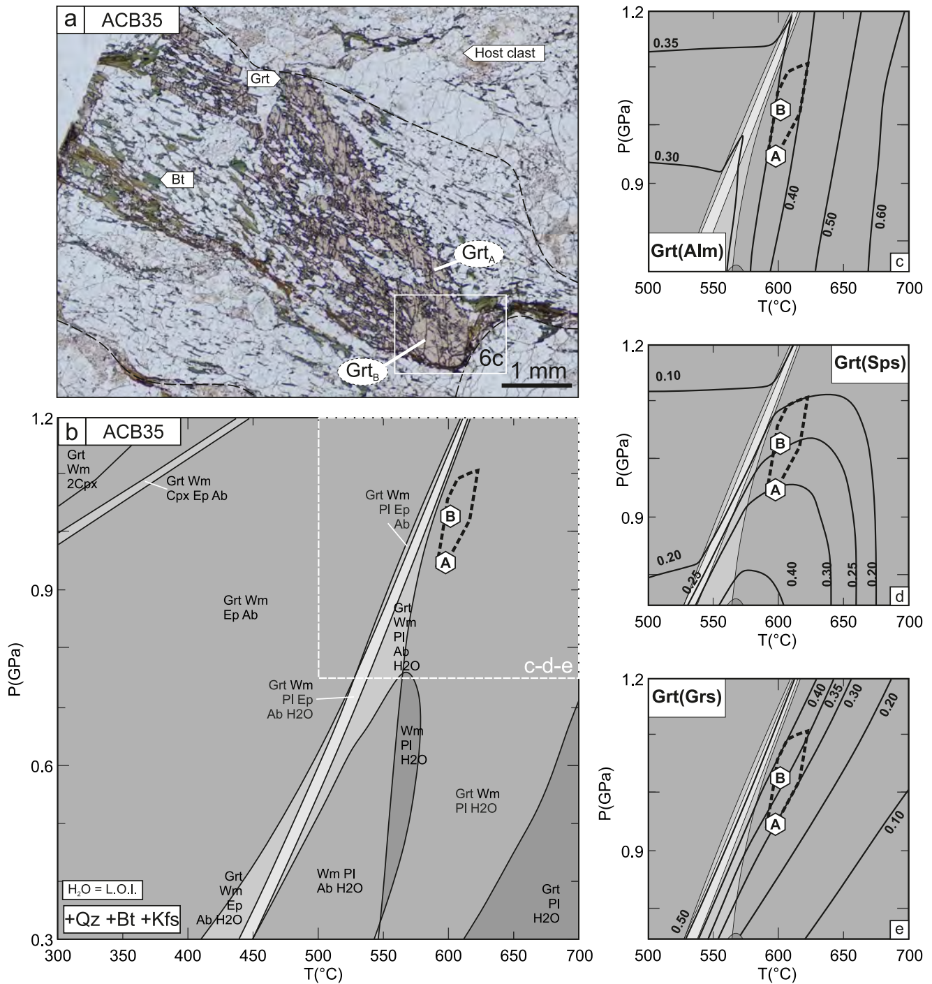
Figure 7. Microstructure and results of pseudosection calculation for sample ACB35—D 1 breccias. (a) Optical plane-polarized light micrograph of the recrystallized matrix of a D 1 breccia (sample ACB35), showing the analyzed honeycomb Grt. (b) Computed pseudosections for sample ACB35. (c–e) Simplified sketch of the pseudosection in panel (b) showing the isopleths for each end-member of the garnet solid solution: (c) Grt(Alm)—almandine, (d) Grt(Sps)—spessartine, (e) Grt(Grs)—grossular. Exagons marked by A and B represent the P - T conditions of stability of Grt A and Grt B compositions reported in the text.
