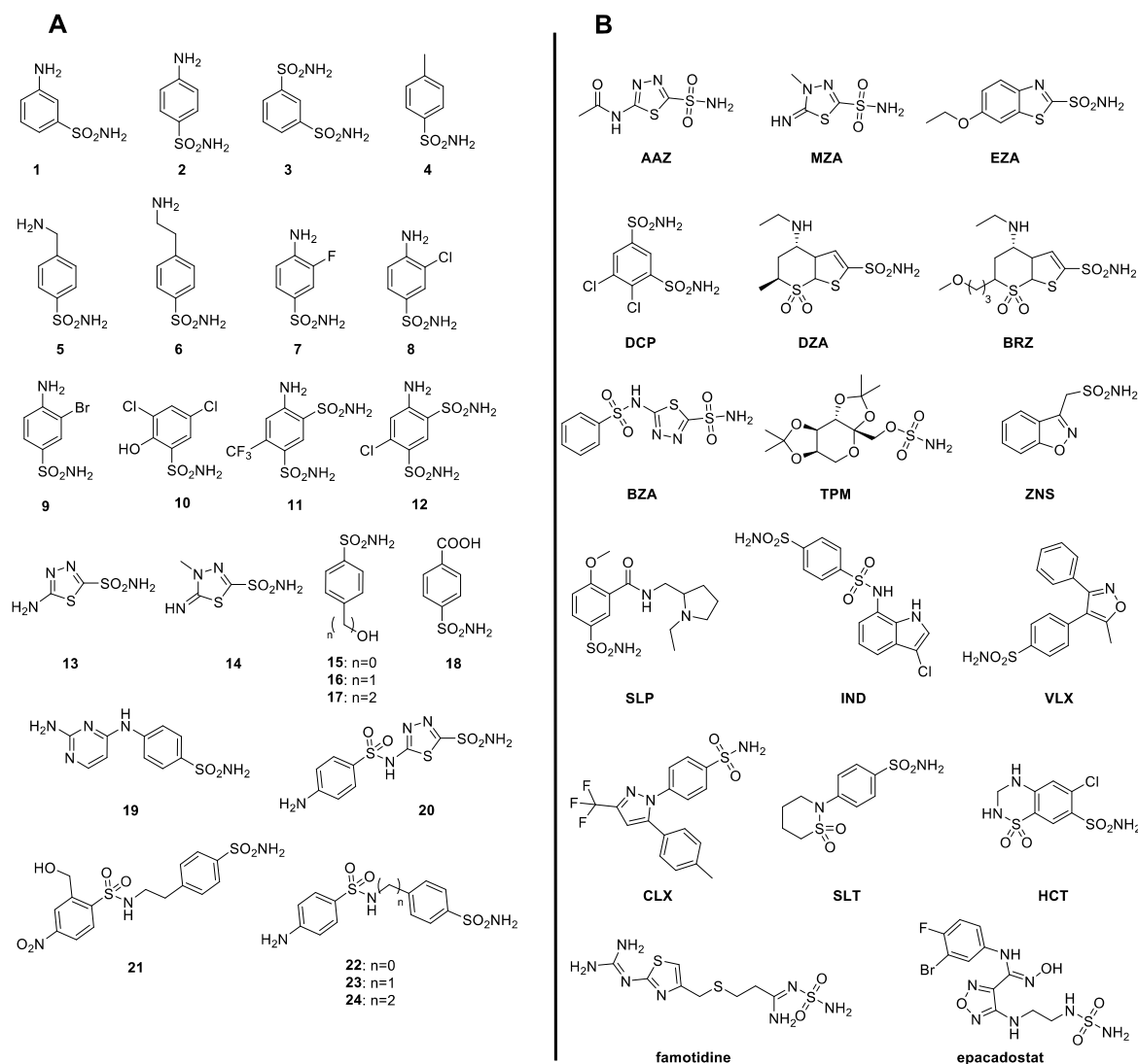
Fig. 3. A. Molecular structures of selective CAIs including sulfonamides and their bioisosteres. B. Molecular structures of AAZ-EPA series of clinically employed for the management and treatment of various diseases and tested for inhibition of SdoCA.
