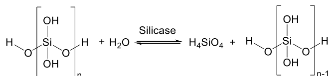
Scheme 2. Reaction catalyzed by SdoCA silicase.
