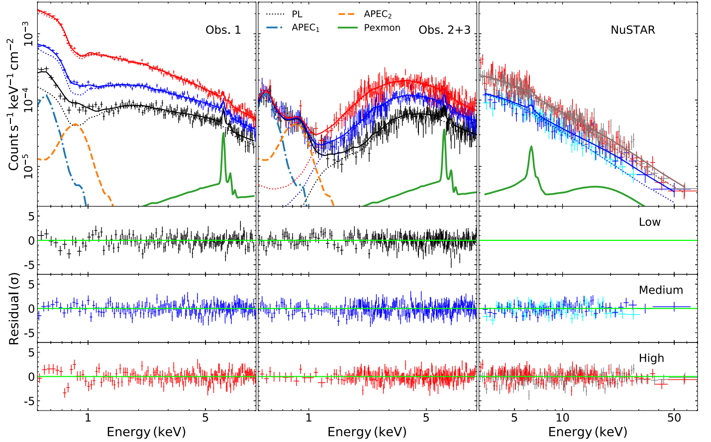
Figure 7. Top panel: spectra and best-fitting model (M3) for all observations. The black, blue, and red spectra in each panel correspond to the low-, medium-, and high-flux spectra, respectively. The blue/cyan and the red/gray NuSTAR spectra correspond to the medium- and high-flux FPMA/B spectra, respectively. The thin dotted lines represent the transmitted power-law component. The thick green lines represent the reflection component, the blue dash-dotted lines and the orange dashed lines correspond to the soft diffuse thermal emission components. Bottom panels: corresponding residuals for each flux level.
