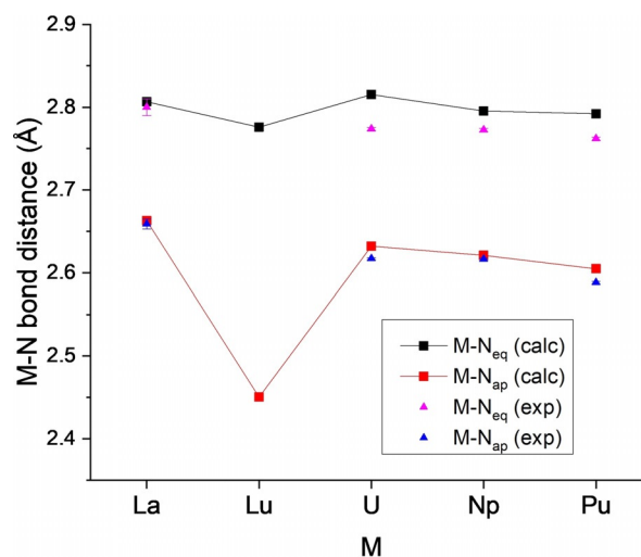
Figure 3. Comparison of computed and available experimental Ln–N (La, Lu) and An–N (U, Np, Pu) bond length. The error bars correspond to the reported experimental uncertainties.
