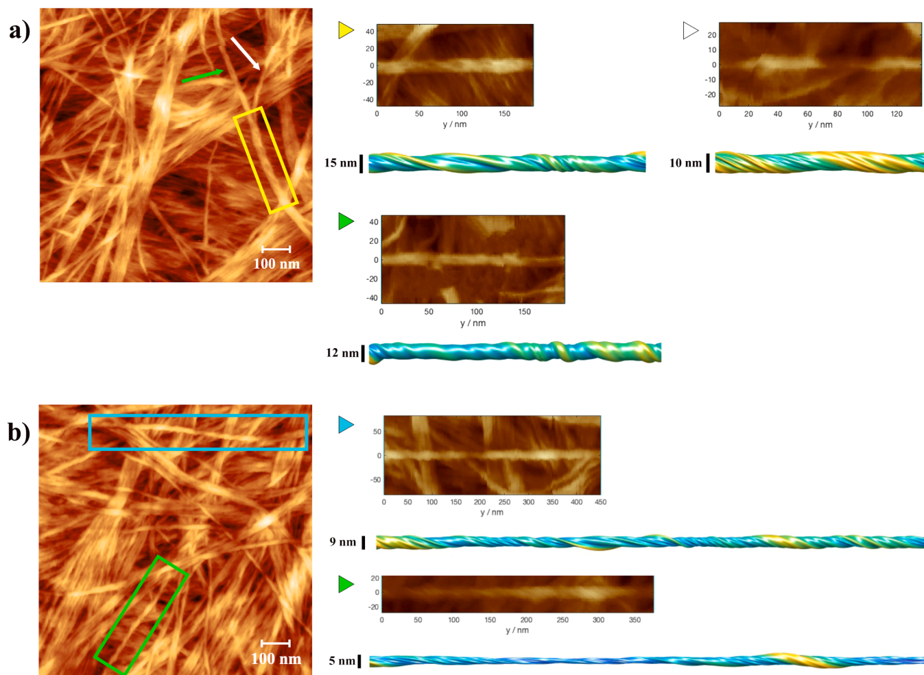
Fig. 4. Two AFM images of the same \text{TFA}^- sample (panels a and b), with arrows and rectangles marking the traced fibrils. To the right of each topographic image, the corresponding straightened fibril is shown above and its 3D reconstruction with its cross-sectional diameter below. Color-coded triangles identify each fibril on the AFM image.
