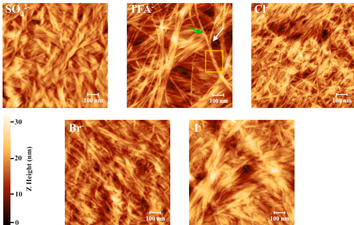
Fig. 3. AFM images of each ACP(65–74)-NH 2 sample containing different counterions. Relative counterions are indicated on each panel.
