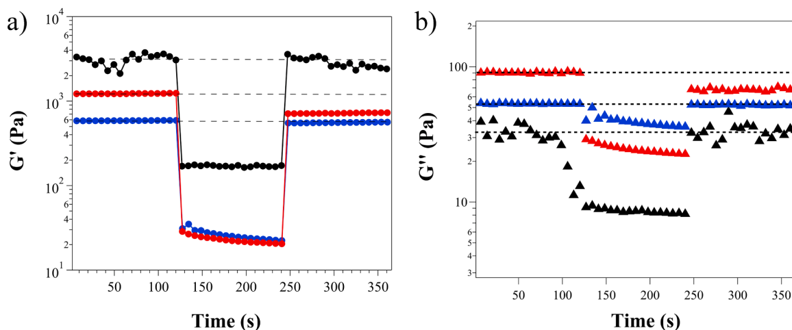
Fig. 8. Three interval thixotropy test (3ITT) results for ACP(65–74)- \text{NH}_2 gels in the presence of \text{TFA}^- (black), \text{Cl}^- (blue) and \text{Br}^- (red): (a) storage modulus G' and (b) loss modulus G'' . The dotted lines serve as guides for the eye.
