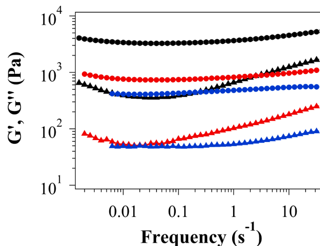
Fig. 7. Frequency sweeps of ACP(65–74)-NH 2 hydrogels in the presence of TFA − (black), Cl − (blue) and Br − (red). The values of G' (circles) and G'' (triangles) are shown for each sample. The experimental error is 3% on each curve.
