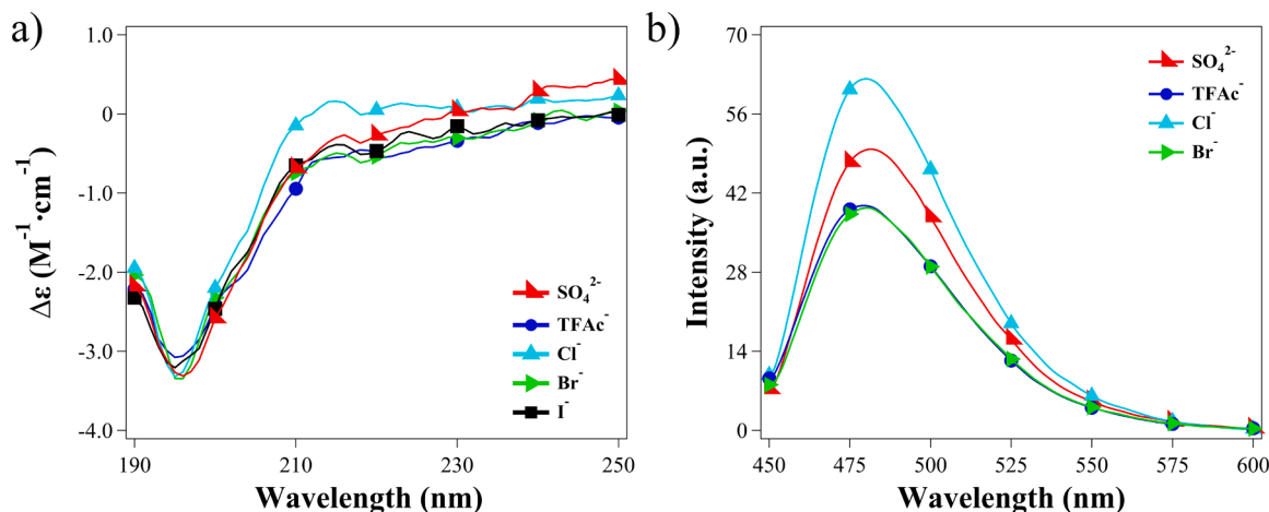
Fig. 6. (a) CD spectrum of ACP(65–74)-NH 2 and (b) ThT fluorescence emission of ACP(65–74)-NH 2 aqueous dispersions at 0.01% w/v concentration in the presence of different counterions.
