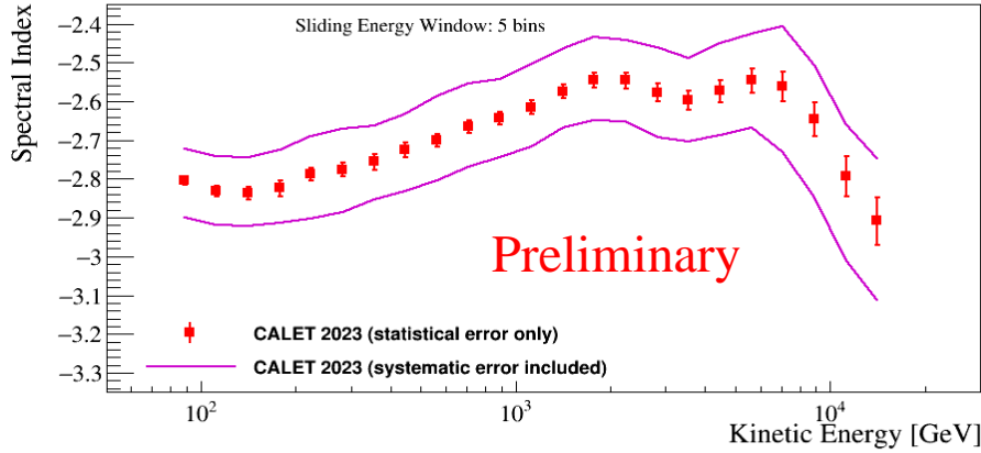
Figure 6: Energy dependence of the spectral index calculated within a sliding energy window for CALET (red square). The spectral index is determined by fitting the data using 5 energy bins (the current bin \pm 2 side bins within errors). The magenta lines show the uncertainty range including systematic errors.
