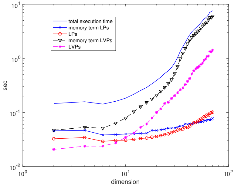
Figure 3: Execution times of Algorithm 1 for solving problem (53) with y(5) given, for dimensions ranging from 2 to 70. See the text for details.
