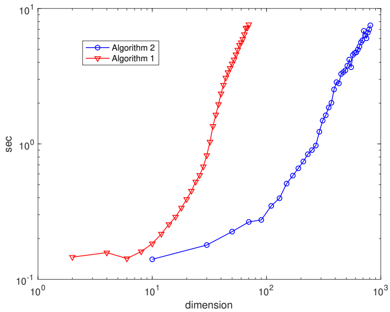
Figure 4: Comparison of the total execution times of Algorithm 1 and Algorithm 2 for solving problem (53) with y(5) given. See the text for details.
