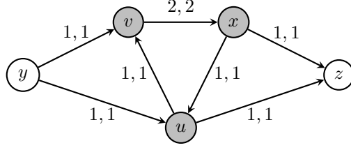
Figure 2: The Flow Decomposition Theorem
