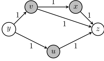
Figure 3: The network N
