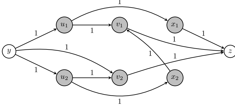
Figure 5: \lambda_{yz}^N(X) > \varphi_{yz}^N(X) for X = \{x_1, x_2\}
