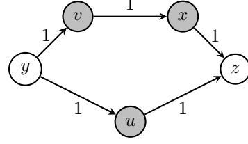
Figure 4: The network N'
