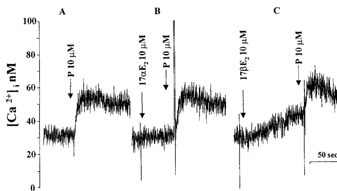
FIG. 4. Effects of 17\alpha E_2 on basal sperm [Ca^{2+}]_i and on calcium response to P. Intracellular calcium waves, in response to P ( 10 \mu M /L) alone (A) and after a previous challenge with 10 \mu M /L 17\alpha E_2 (B) or 17\beta E_2 (C), are shown. Note that 17\alpha E_2 does not affect either basal or P-stimulated [Ca^{2+}]_i . Results are representative of three similar experiments.
