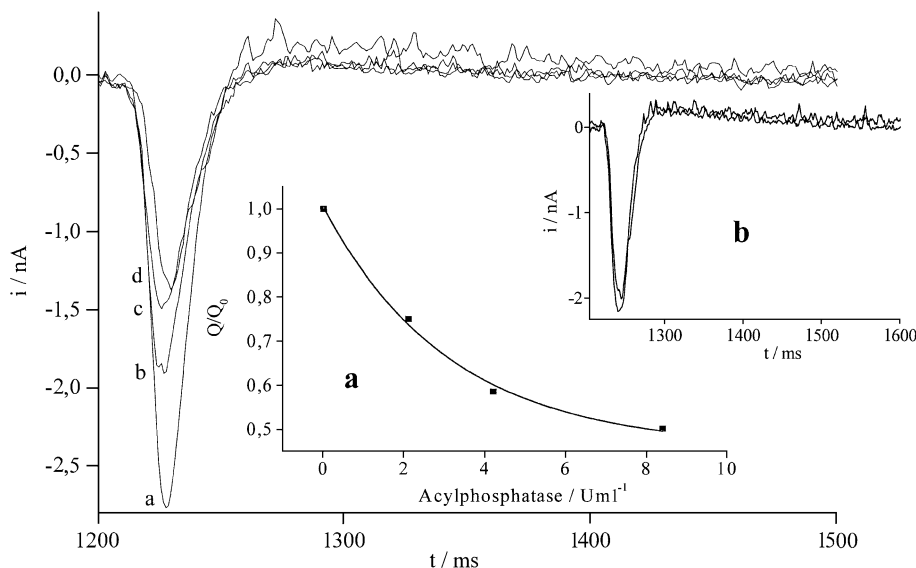
Fig. 4. Current transients generated by \text{Na}^+, \text{K}^+ -ATPase following 100 \mu\text{M} ATP concentration jumps in the presence of varying amounts of AcP: 0 (a), 2.1 (b), 4.2 (c) and 8.4 U/ml (d), corresponding to 0, 2.3, 4.6 and 9.2 \mu\text{g/ml} of AcP. The AcP concentration was the same in both the nonactivating and the activating solution. Both solutions also contained 130 mM NaCl, 25 mM imidazole, 3 mM \text{MgCl}_2 and 0.2 mM DTT at pH 7.0 (HCl). Inset (a) shows the ratio of the charge Q translocated in the presence of AcP to that, Q_0 , translocated in its absence against the AcP concentration. Inset (b) shows the current transients following 100 \mu\text{M} ATP concentration jumps in the presence and absence of the AcP mutant N41S. The concentration of the mutant in both the activating and nonactivating solutions was equal to 9.2 \mu\text{g/ml} and equivalent to 8.4 U/ml of active AcP. Both solutions also contained 130 mM NaCl, 25 mM imidazole, 3 mM \text{MgCl}_2 and 0.2 mM DTT at pH 7.0 (HCl).
